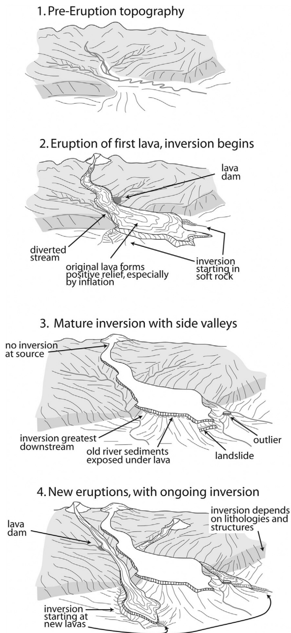
Fig. 1. Sketch explaining the progressive development of inversion. A. Original topography. B. Topography after first eruption catastrophically changes drainage, creating relief and erosion immediately starting the process of inversion. C. Mature inversion created by long term erosion, with differential rates on different lithologies, across structures. D. New eruptions suddenly change the drainage system and reset the inversion process, that resumes immediately.
