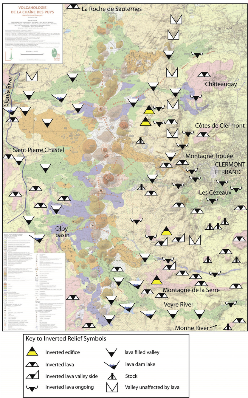
Fig. 12. Map of the Chaîne des Puy - Limagne fault area (Auvergne, France) showing different types of inverted relief using a pictogram symbolism. This illustrates the great diversity of inverted relief elements around this area.
