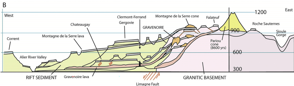
Fig. 11. Scrope's (1827) schematic cross sections of the inverted relief over the Limagne fault and Mont Mezen near le Puy en Velay (Auvergne, France). A. A copy of the original diagram, which is one of the first descriptions of inverted relief in landscape evolution. B. Modern copy drawn to show clearly the profiles of the inverted relief lavas to the east and west of the Chaîne des Puys volcanoes, and the Limagne fault.
