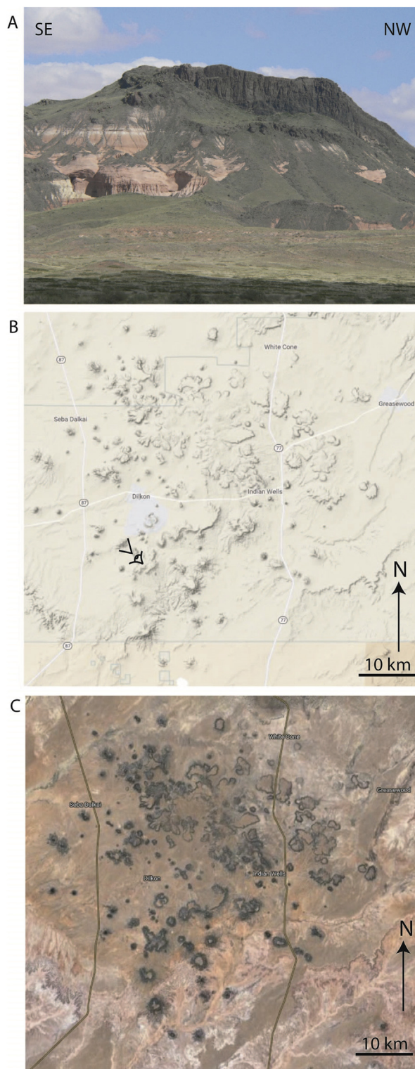
Fig. 20. Hopi Buttes (Arizona). A. Photo of the Castle Hill, a mesa with a flat lava cap (photo: Dávid Karatson). B. Google Map extract showing the relief and C. Google Earth satellite image. Note: This eroded volcanic field contains superb, exhumed vents, including shallow intrusions. There are only a few lava flows, that seem to have mostly been erupted on flat topography, and which now form mesas.
