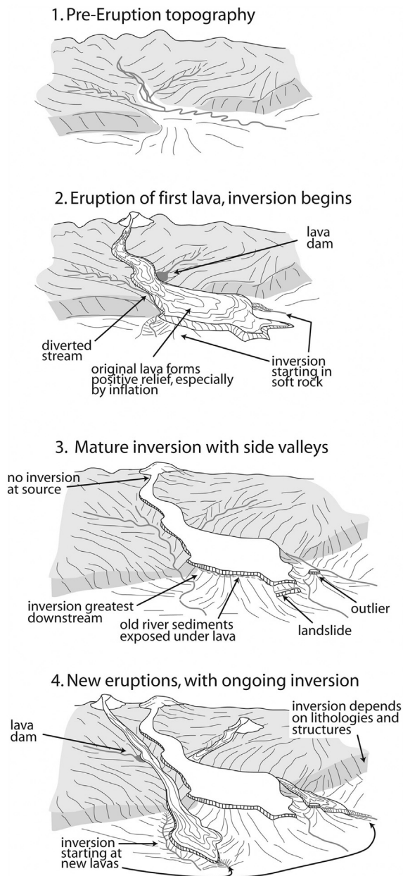
Fig. 1. Sketch explaining the progressive development of inversion. A. Original topography. B. Topography after first eruption catastrophically changes drainage, creating relief and erosion immediately starting the process of inversion. C. Mature inversion created by long term erosion, with differential rates on different lithologies, across structures. D. New eruptions suddenly change the drainage system and reset the inversion process, that resumes immediately.
