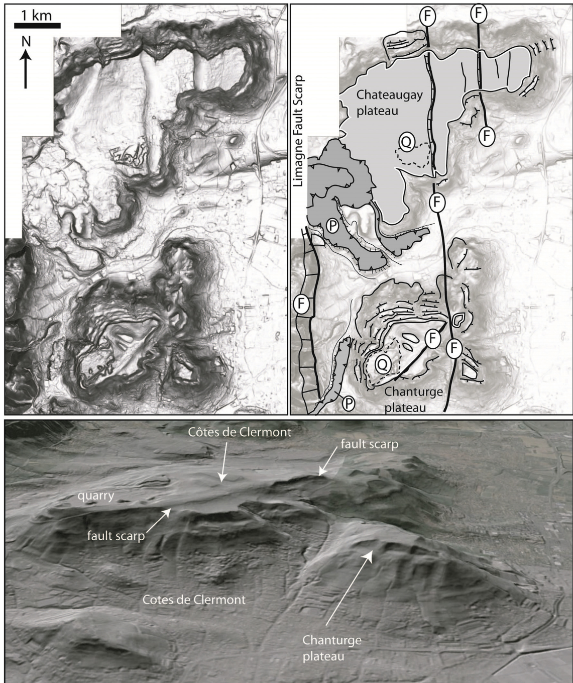
Fig. 8. Inverted relief showing tectonic activity, and additional geomorphological processes. A. LIDAR image in shaded relief of the Chateaugay and Chanturges plateaux (Auvergne, France), next to the Limagne fault. B. Annotated map showing inverted relief and faults. The Chateaugay lava is cut by two prominent normal faults (F); the Chanturges plateaux's east side is also cut, but landslide blocks confuse the faulting pattern. Many landslides are visible around the plateaux. Several recent lavas have descended to the plain, flowing around the inverted relief. These flows (P) are also beginning to be inverted. Data from the CRAIG database (Lidar Clermont). C. Oblique shaded relief image of Chanturges and Cotes de Clermont. Image shows the outlying mesa (Chanturges), and the main plateau, with a north-east trending fault scarp downthrowing the plateau.
