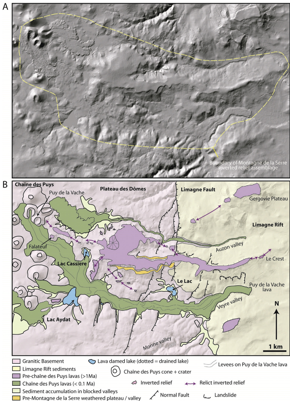
Fig. 13. Montagne de la Serre (Auvergne). A. Shaded relief image of the area. B. Map of the main features, the older and younger lavas, blocked valleys, recent inversion, and relict inversion etc.
