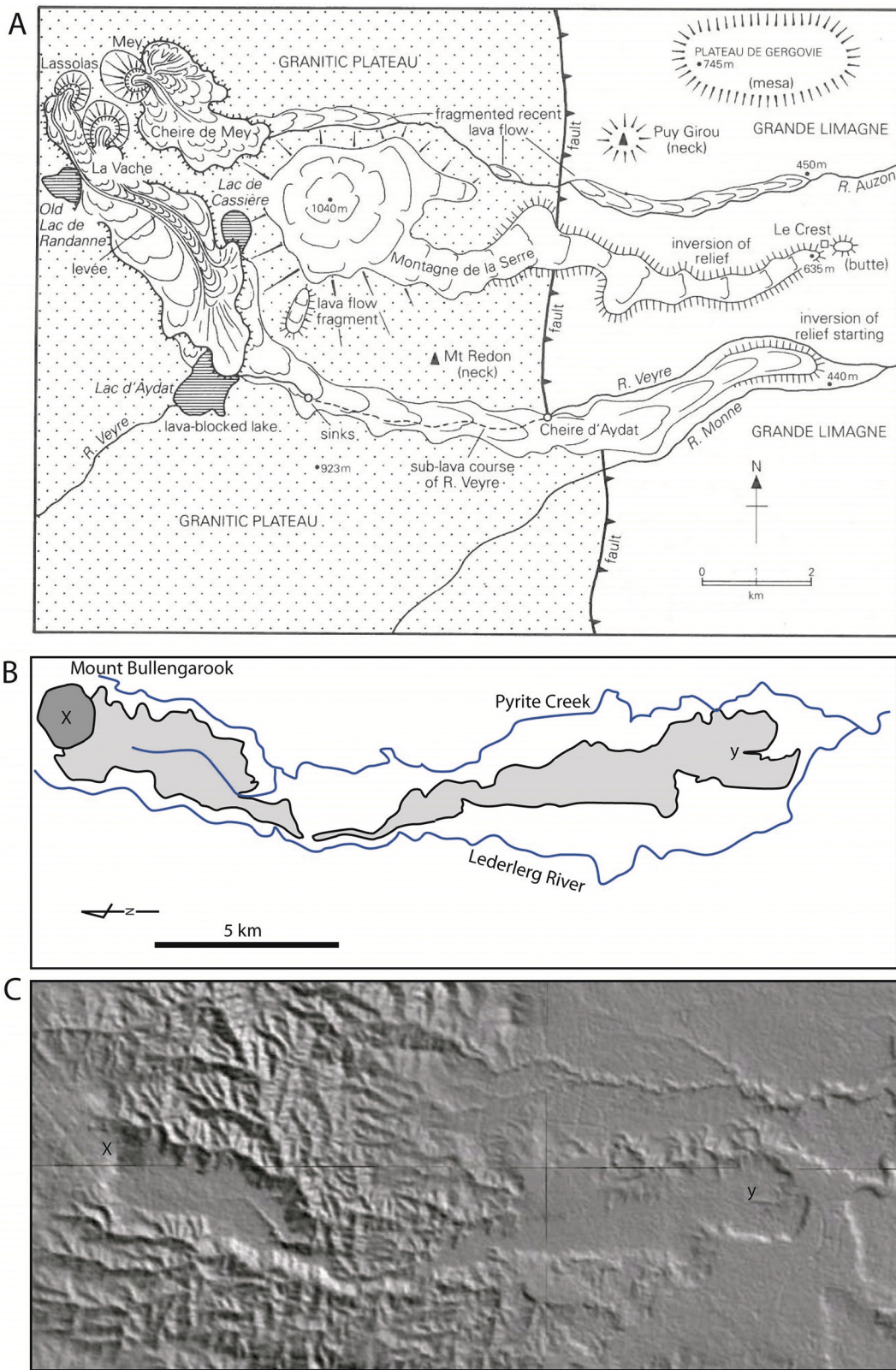
Fig. 10. Classic examples of inverted relief. A. Scarth's 1966 sketch map of the Montagne de la Serre area (Auvergne). B. A redrawn version of Pain and Ollier's (1995) map of the Mount Bullengarook lava flow inversion (Southeast Australia). C. Shaded relief image of the STRM 30 m digital terrain model showing the relief of the Bullengarook lava.
