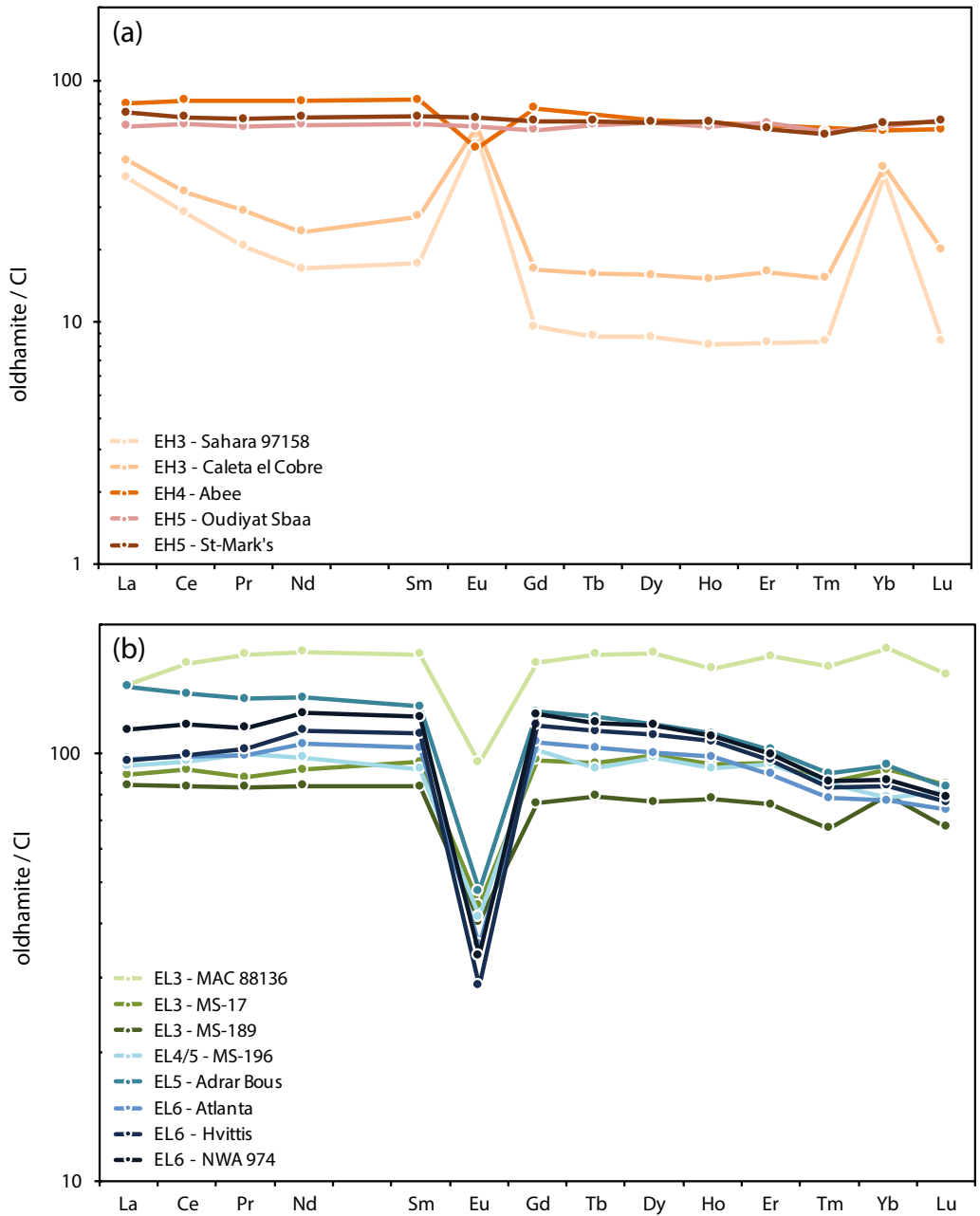
Fig. 4 CI-normalized REE abundances in oldhamites from EH chondrites (a) and EL chondrites (b). CI values are from Barrat et al. (2012)
