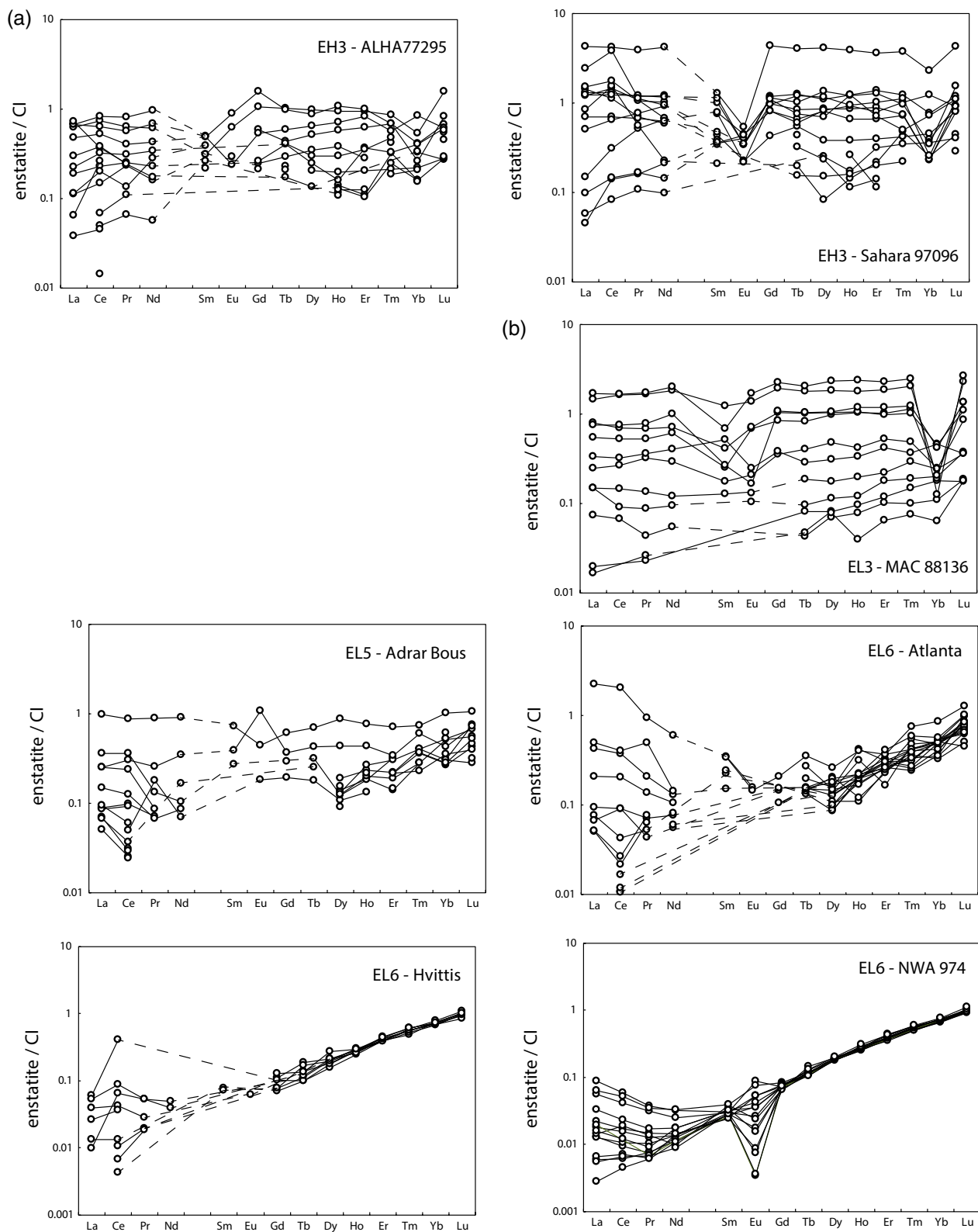
Fig. 5 REE patterns of enstatite in EH (a) and EL (b) chondrite. CI values are from Barrat et al. (2012)
