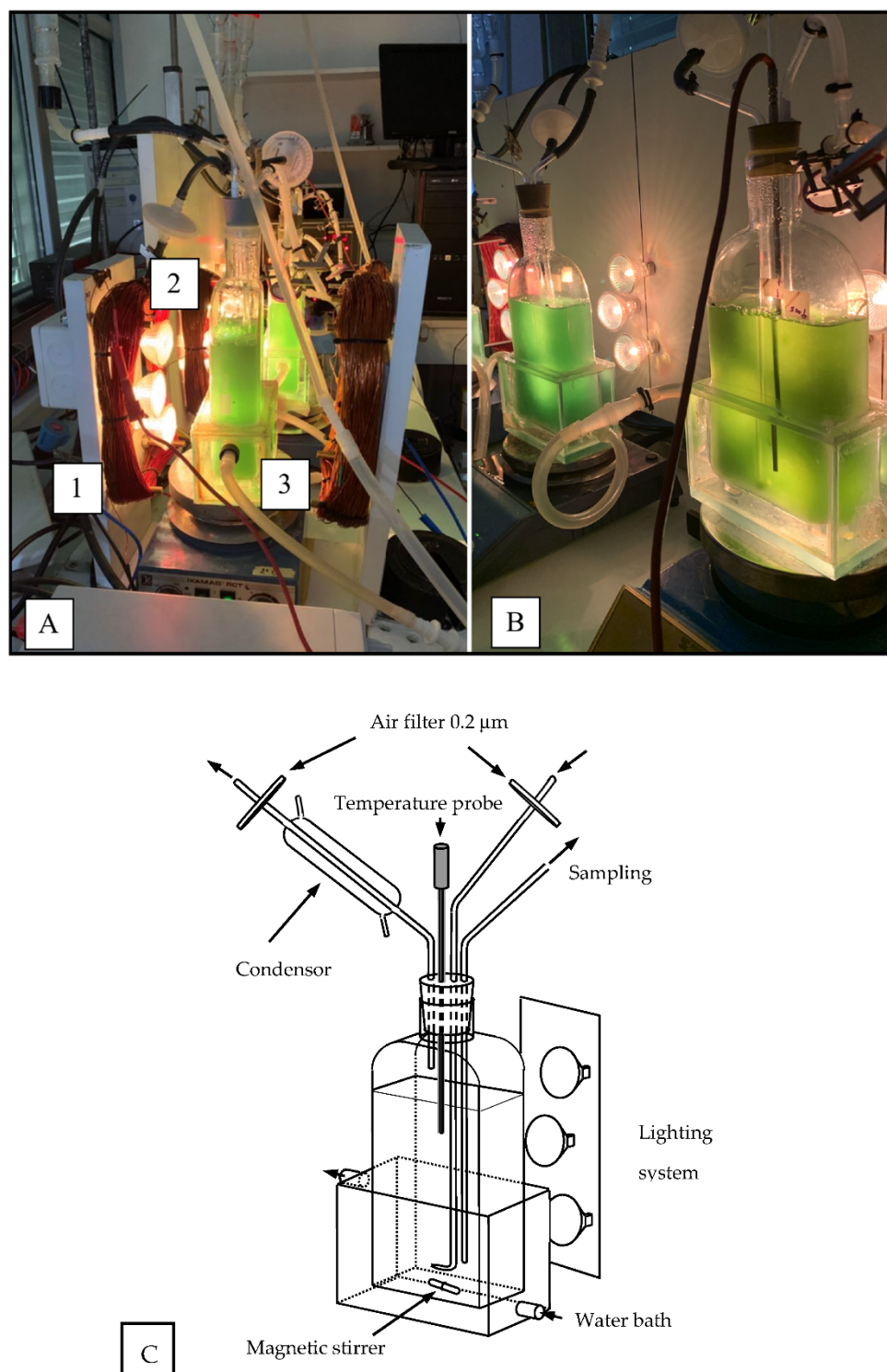
Figure 1. Experimental device used for the L. indica PCC8005 cultivation. (A) Cultures with magnetic field application through coils and (B) cultures control without MF application but in the same temperature, luminosity and aeration conditions. (1) Coils with 400 turns used to generate the MF, (2)
