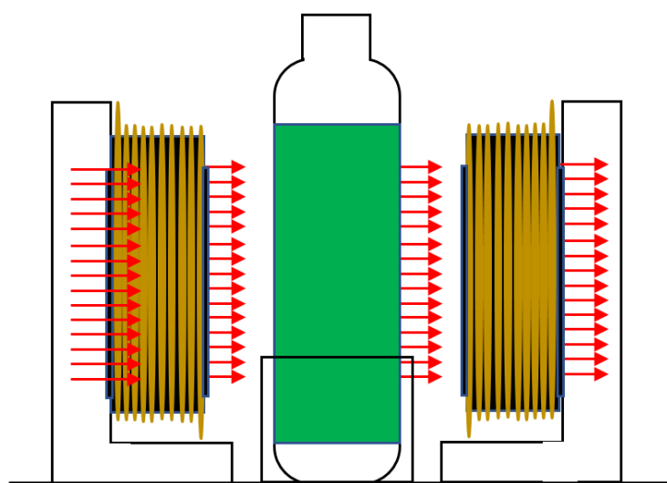
Figure 2. Schematic diagram of the experimental device used for the L. indica PCC8005 cultivation with magnetic field application through coils. Red arrows indicate the transverse magnetic field.
