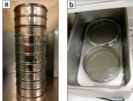
Fig. S3. Sieving and cleaning the sieves. (a) Column of full- \phi sieves from -4 \phi to +4 \phi . A column of half- \phi sieves will yield a more detailed grainsize distribution. (b) Cleaning the finer sieves in an ultrasonic bath, after each sample is sieved.
