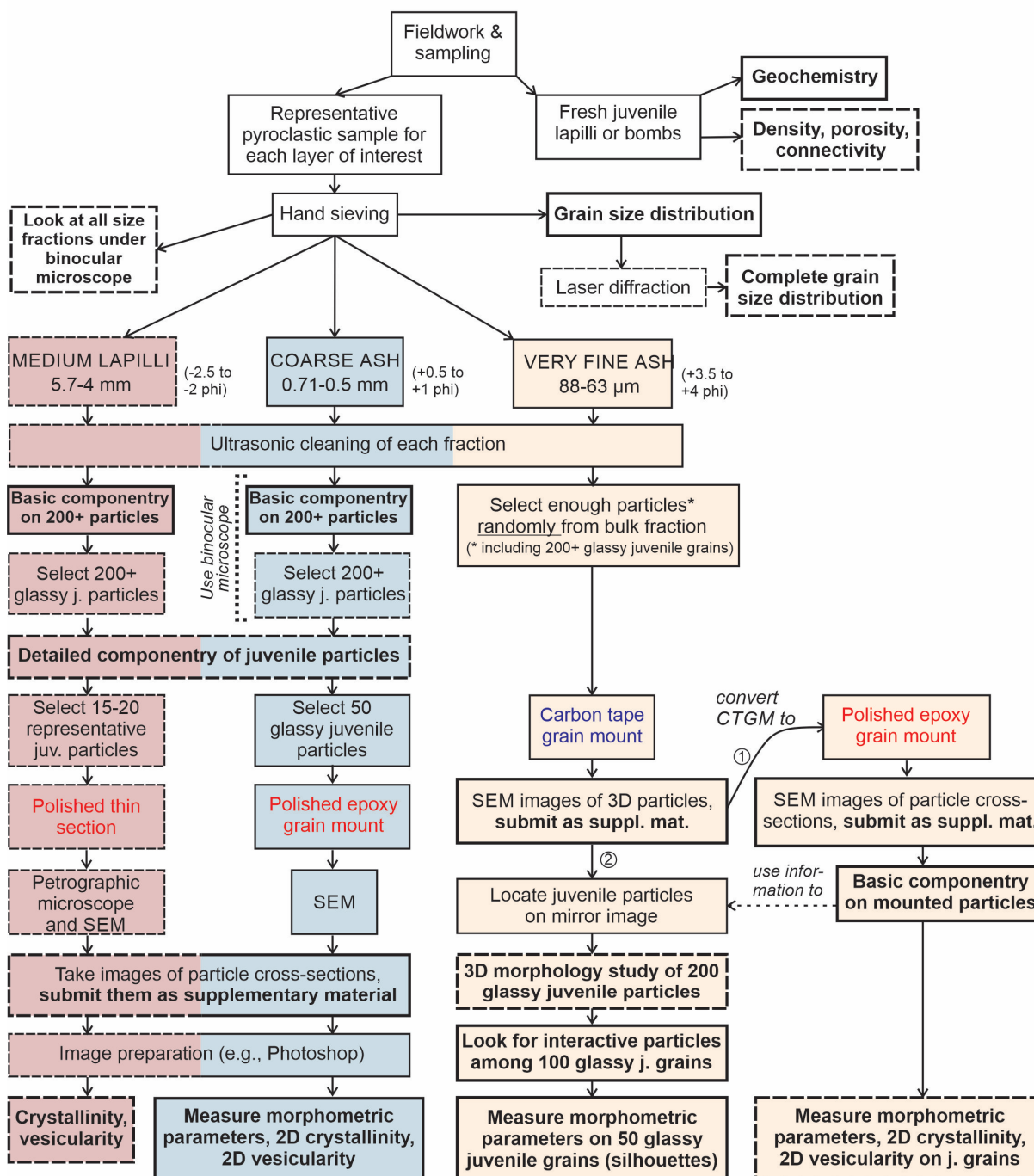
Fig. 2. Flowchart of the steps needed to analyze juvenile pyroclasts for comparative fragmentation studies, showing standard steps (continuous lines) and recommended steps (dashed lines). Bold items are outputs.
