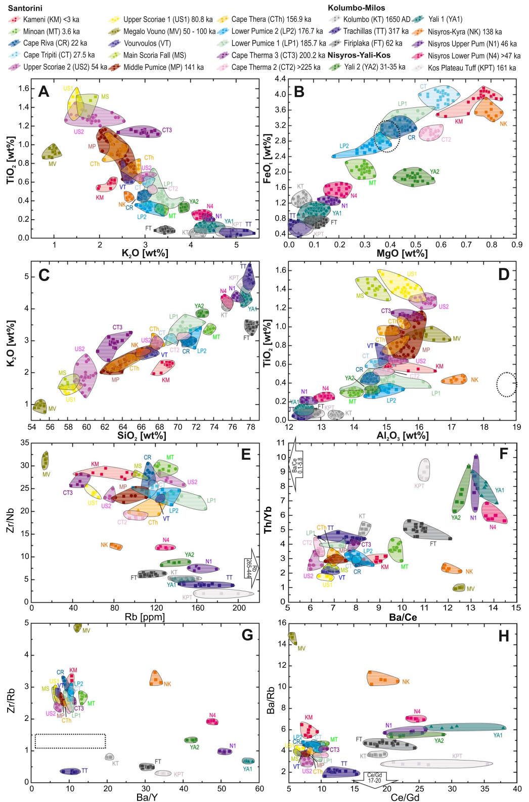
Figure 6. Matrix-glass compositional ranges of proximal onshore tephras (normalized to 100 wt% anhydrous compositions). Colored areas represent the correlation fields, dashed boxes enclose the single measurements. See data in supplementary tables in Data Set S1.
