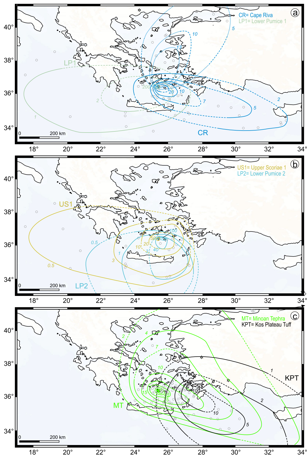
Figure 7. Isopach maps for four widespread Santorini tephra. Italic numbers on isopachs indicate thickness in centimeters. (a) Cape Riva Tephra (CR) and Lower Pumice 1 (LP1). (b) Upper Scoriae 1 Tephra (US1) and Lower Pumice 2 (LP2). Data source and other features as on Figure 5. Several cm thick tephra from Cape Riva have also been found in Tenaghi Philippon (Seymour et al., 2004; Wulf et al., 2018), in the southwestern Black Sea (Kwiecien et al., 2008), and in western Turkey (Roeser et al., 2012). The data points have been considered for the isopachs and volume estimates but lie outside the map area.
