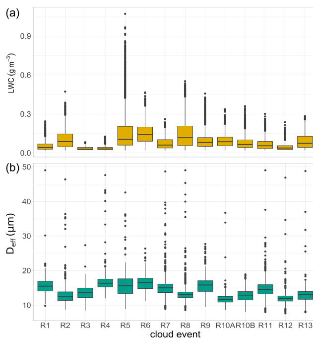
Figure 2. Distribution of liquid water content (LWC) and effective diameter ( D_{\text{eff}} ) of cloud droplets observed during each cloud event in Réunion. R1 to R13 refer to individual cloud samples. Lower and upper box boundaries represent the 25th and 75th percentiles, respectively; line inside box shows the median, and lower and upper error lines depict the 10th and 90th percentiles, respectively; filled black circles represent the data falling outside the 10th and 90th percentiles.
