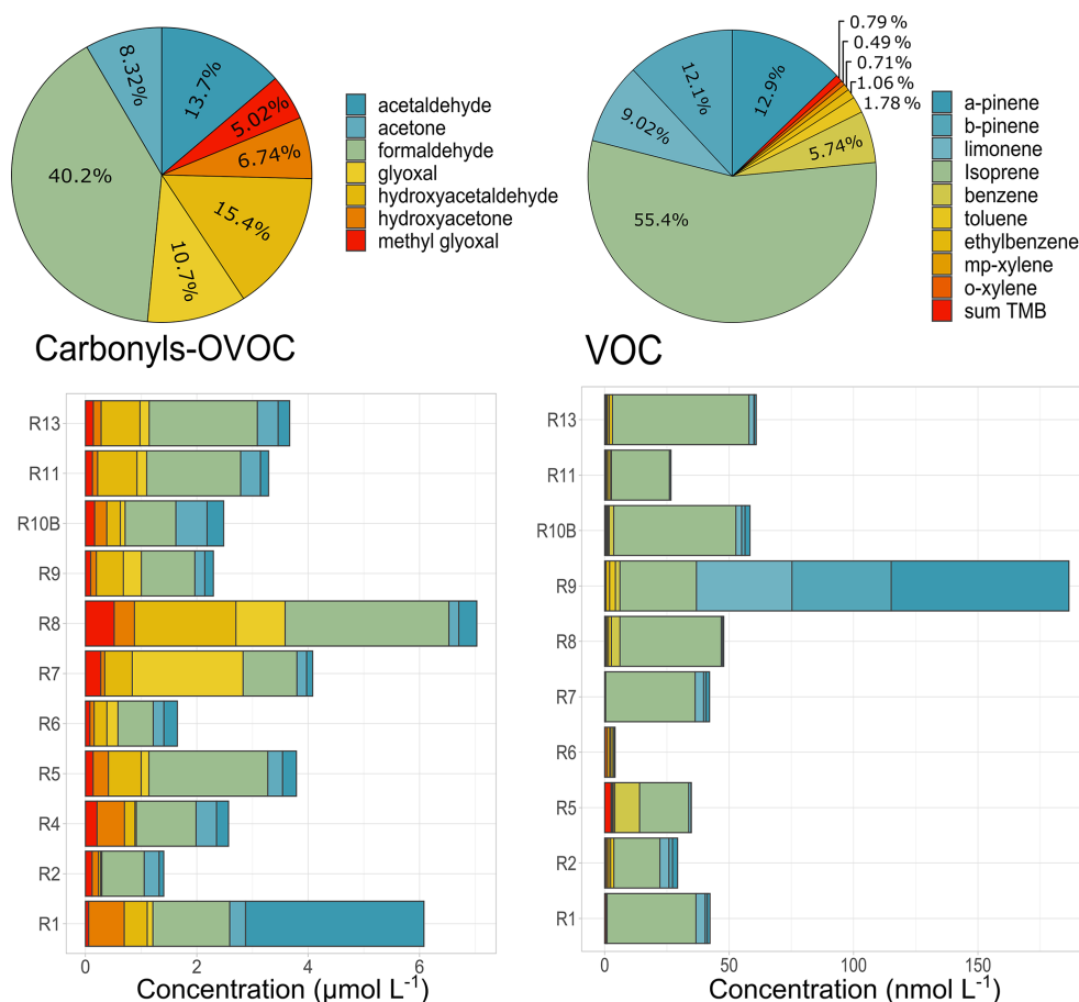
Figure 6. Concentrations and total relative contributions of carbonyls ( \mu\text{molL}^{-1} ) and low-solubility VOC ( \text{nmolL}^{-1} ) species observed in cloud waters. Sum TMB represents the sum of 1,2,4-trimethylbenzene, 1,3,5-trimethylbenzene, and 1,2,3-trimethylbenzene concentrations. R1 to R13 refer to individual cloud samples.
