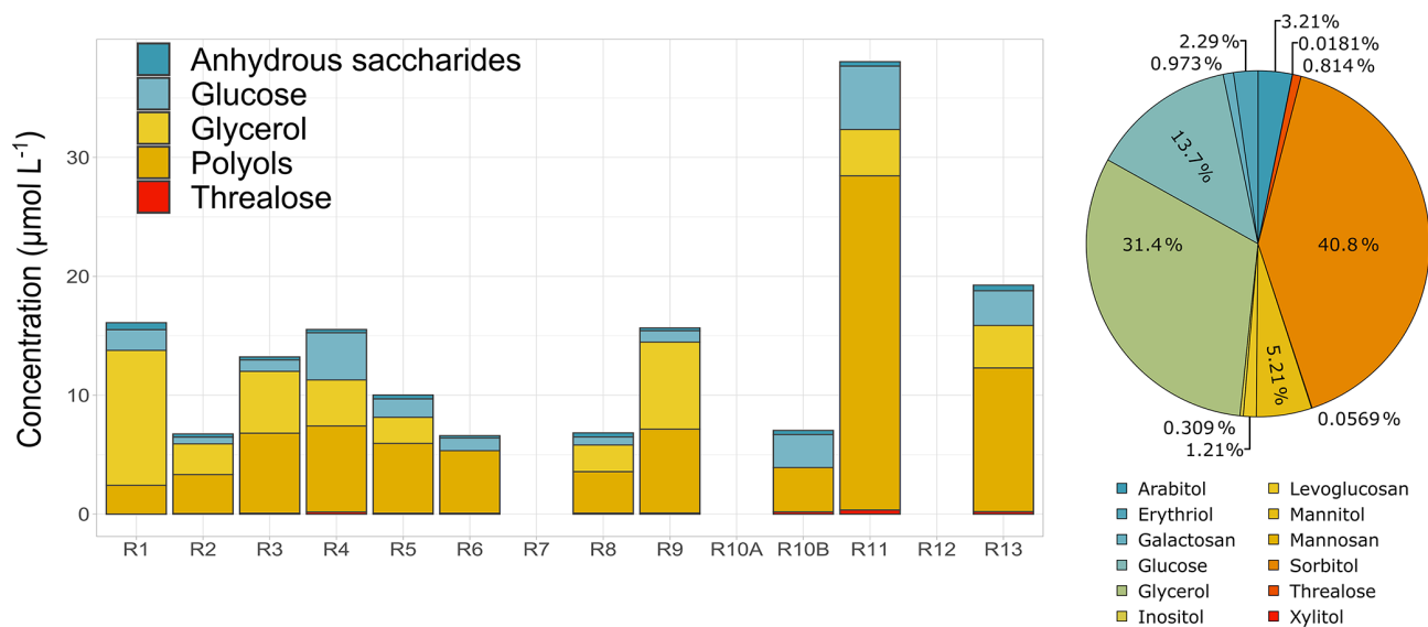
Figure 5. Concentrations of polyols, anhydro saccharides, and monosaccharides and total average relative contributions of sugars observed in cloud waters. R1 to R13 refer to individual cloud samples.
