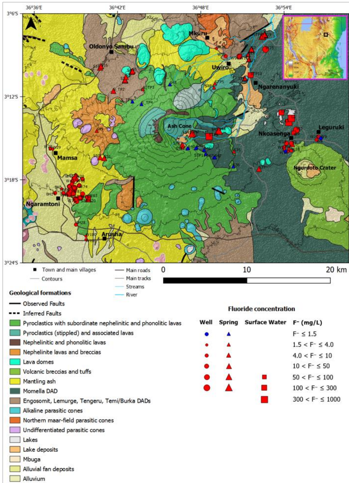
Fig. 1. Geological map of the study area adapted from Bennett et al. (2021), indicating different geological formations and spatial distribution of F - concentrations of sampled water points. A small map inserted in the top right corner is the map of Tanzania (modified after Mapsland (2021), the original image is under Creative Commons Attribution-ShareAlike 3.0 Unported (CC BY-SA 3.0) license), showing the location of Mount Meru using a black lined square box.
