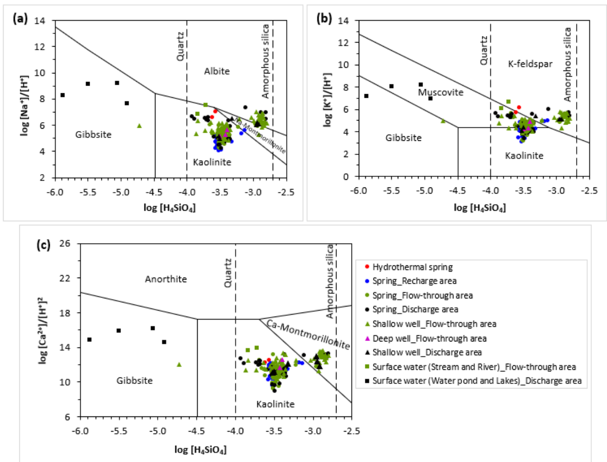
Fig. 9. a to c: Stability diagrams of Na-, K- and Ca-feldspars and its weathering products for groundwater samples from the study area. The dashed lines represent saturation with respect to quartz and amorphous silica.
