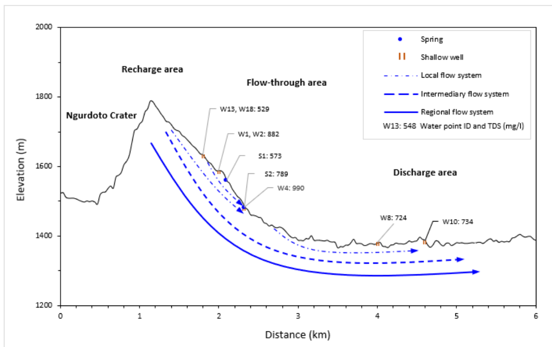
Fig. 3. Simplified groundwater flow conceptual model for the northern flank of Ngurdoto crater showing the increase of groundwater mineralisation with water residence times.
