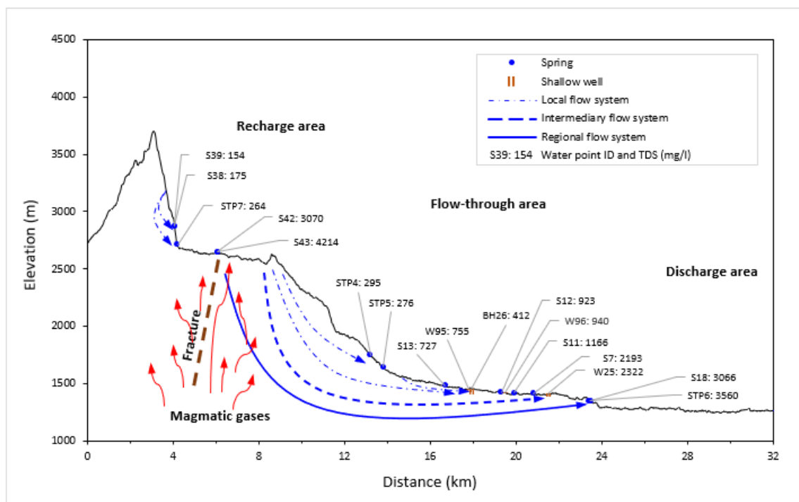
Fig. 2. Simplified groundwater flow conceptual model for the north-eastern flank of Mount Meru adapted from Bennett et al. (2021), suggesting the influence of the volcanic gases in the groundwater chemistry and also showing the increase of groundwater mineralisation with water residence times.
