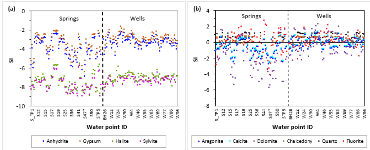
Fig. 6. a to b: Saturation index (SI) of potentially relevant minerals for the groundwater samples.
