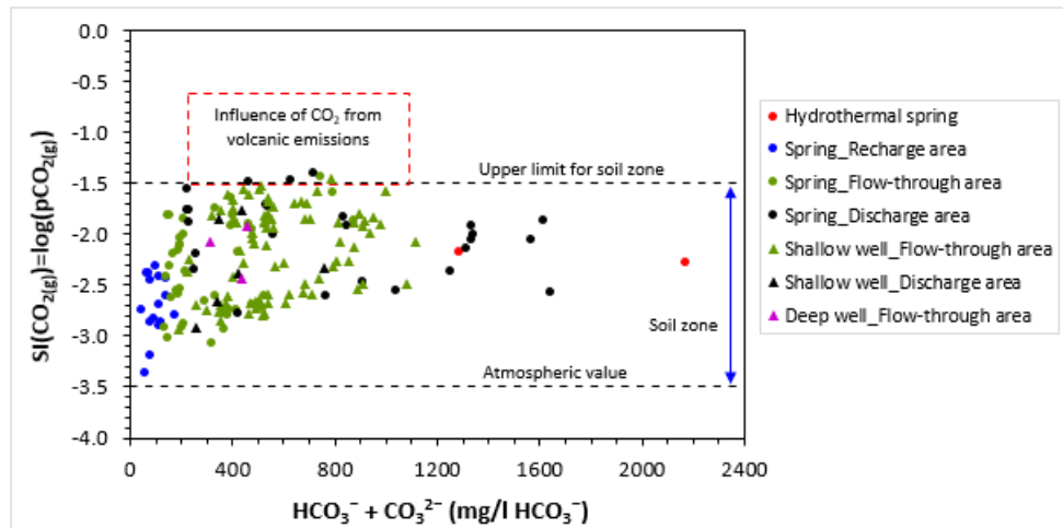
Fig. 7. Relationship between \text{HCO}_3^- + \text{CO}_3^{2-} and \log(p\text{CO}_{2(g)}) for the groundwater samples.
