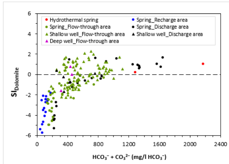
Fig. 15. Bivariate plot of saturation index (SI) of dolomite versus \text{HCO}_3^- + \text{CO}_3^{2-} in groundwater samples.
