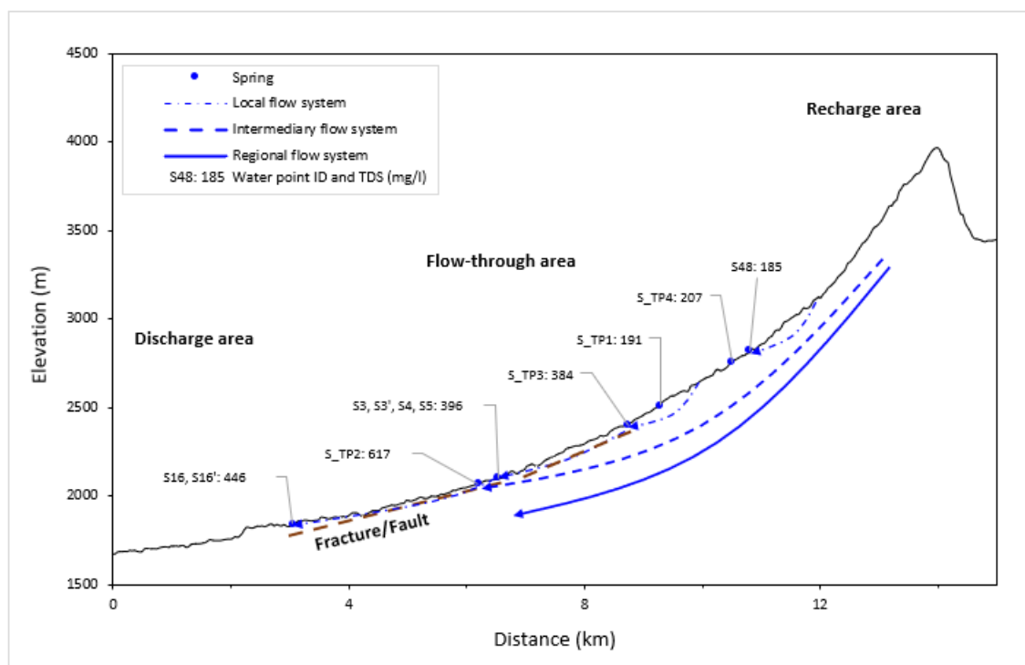
Fig. 4. Simplified groundwater flow conceptual model for the north-western flank of Mount Meru showing the increase of groundwater mineralisation with water residence times.
