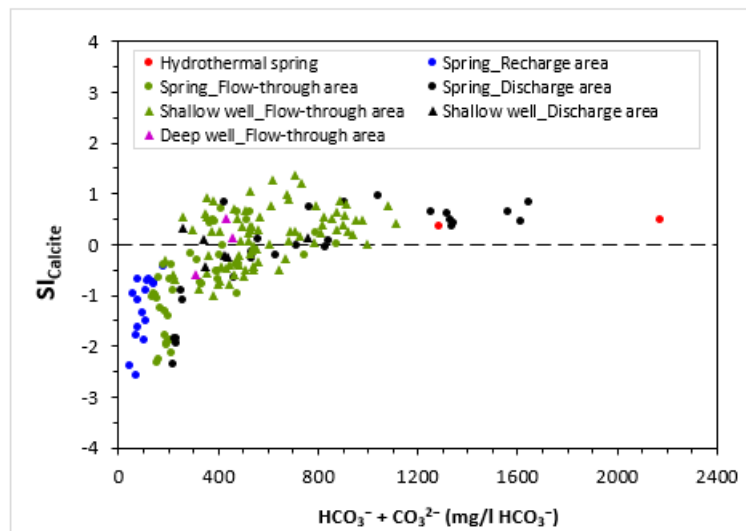
Fig. 12. Bivariate plot of saturation index (SI) of calcite versus \text{HCO}_3^- + \text{CO}_3^{2-} in groundwater samples.
