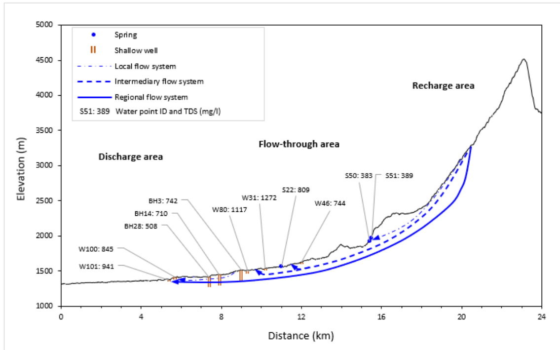
Fig. 5. Simplified groundwater flow conceptual model for the south-western flank of Mount Meru showing the increase of groundwater mineralisation with water residence times.
