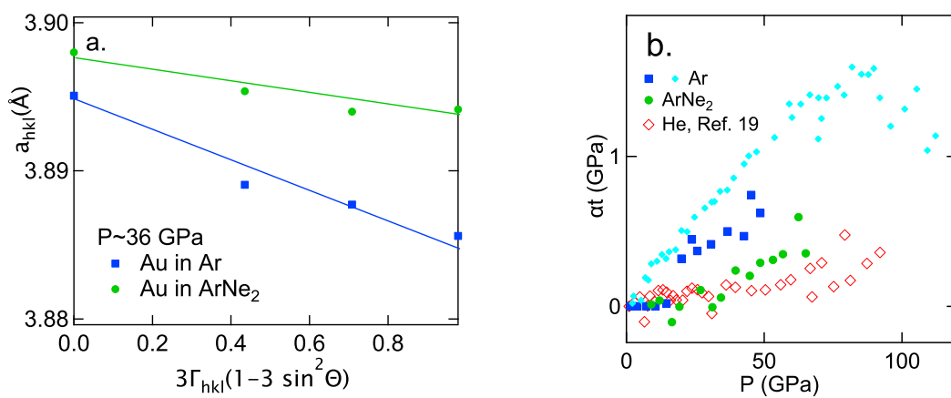
Figure 6. Evaluation of non-hydrostatic stress in runs 1 and 2 based on Au X-ray diffraction lines position. a. Gamma plot for Au around 36 GPa. In this plot and underlying model, the slope of a_{hkl} vs 3 \times \Gamma_{hkl} \times (1 - \sin^2 \theta) is proportional to uniaxial stress t in Au. b. \alpha t ( \alpha \sim 0.5 ) estimated with this analysis, vs pressure, in runs 1, 2 and 4. It is compared to values estimated for Au compressed in He 19 .
