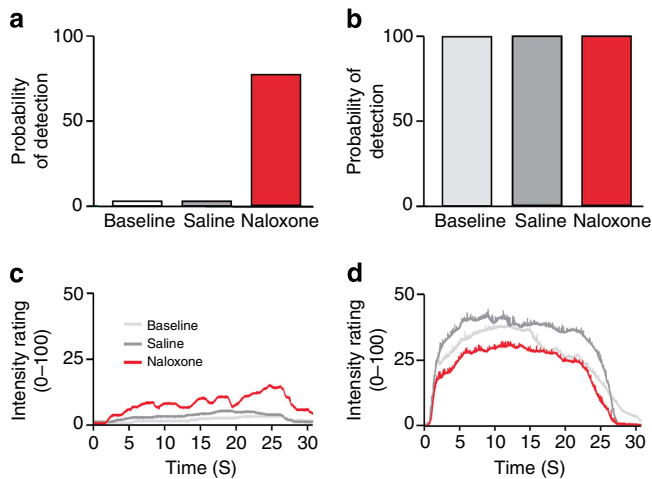
Figure 5 | Naloxone dramatically reverses the analgesia associated with \text{Na}_v1.7 -null mutations in a CIP individual. Perception of phasic pain. The probability of detecting 9-ms radiant heat pulses was assessed in a \text{Na}_v1.7 -null patient (a) and in three age-matched healthy controls (b). Neodymium:yttrium-aluminum-perovskite (Nd:YAP) laser pulses (El.En, Italy) selectively stimulate intra-epidermal free-nerve endings, thus providing a pure nociceptive input without touch. The human \text{Na}_v1.7 null did not detect any stimuli in baseline and saline conditions. The probability of detecting the stimulus dramatically increased to 80% of stimuli detected during the infusion of 12 mg naloxone, almost reaching the detection levels of matched healthy controls. (c,d) Tonic pain was elicited by 25 s laser stimuli, whereas the participants rated online the intensity of the heat sensation on a visual analogue scale (0 = no sensation, 100 = worst pain imaginable) throughout the laser application. Again, naloxone strongly enhanced tonic pain sensations in the \text{Na}_v1.7 -null patient (c) throughout the time course of the stimulation without effect in the control subjects (d).
