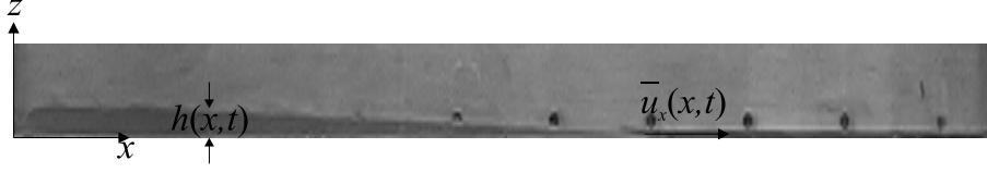
Figure 1: Orientation of axes, and notation associated with modelling the currents. The image shows a fluidised current approximately 65cm long and 2cm thick.
