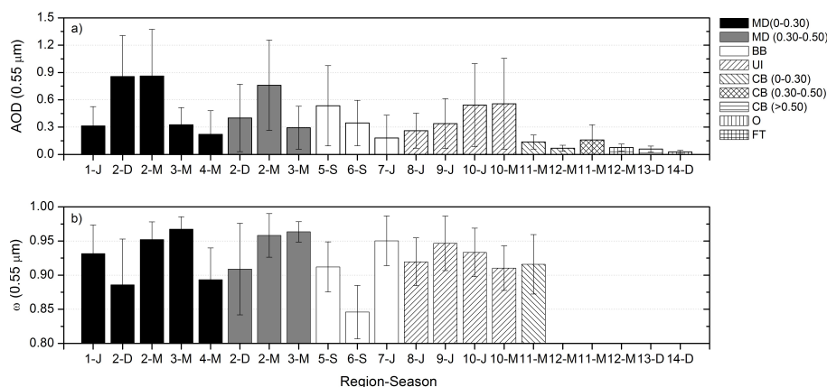
Fig. 5. Multi-year average of aerosol optical depth, AOD, at 0.55 μm (a), and single scattering albedo, \omega , at 0.55 μm (b), for each region and season. M = March–April–May, J = June–July–August, S = September–October–November and D = December–January–February. The legend shows each aerosol type: MD = Mineral Dust, BB = Biomass Burning, UI = Urban–Industrial, CB = Continental Background, O = Oceanic and FT = Free Troposphere. For the regions influenced by desert mineral dust and continental background, the AOD and \omega averages have been evaluated for each interval of surface albedo (SA): 0–0.30, 0.30–0.50 and >0.50. Error bars indicate \pm 1\sigma ( \sigma , standard deviation).
