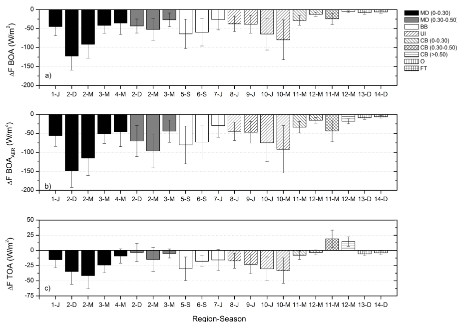
Fig. 6. Multi-year average of the aerosol radiative forcing, \Delta F ( \text{Wm}^{-2} ), at the BOA (Eq. 3) (a), AERONET \Delta F BOA AER at the BOA (Eq. 5) (b), and \Delta F at the TOA (Eq. 2) (c) for each region and season. The seasons and aerosol types are labeled as Fig. 5. Error bars indicate \pm 1\sigma ( \sigma , standard deviation).
