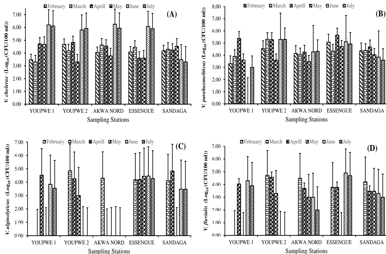
Figure 3. Spatio-temporal variations in cell abundance of Vibrio cholerae (A), Vibrio parahaemolyticus (B), Vibrio alginolyticus (C), Vibrio fluvialis .
