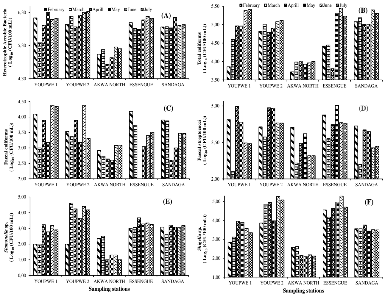
Figure 2. Spatio-temporal variations in cell abundance of Heterotrophic Aerobic Bacteria (A), Total Coliforms (B), Faecal Coliforms (C), Faecal Streptococci (D), Salmonella sp. (E), and Shigella sp. (F)
