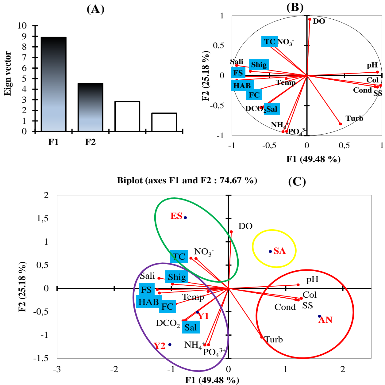
Figure 3. Result of the Principal Component Analysis (PCA) carried out on the physicochemical and bacteriological variables measured in the different stations during the study period: (A) Histogram of the eigen vector; (B) Correlation circle between variables and factorial axes F1 and F2; (C) Biplot showing the distribution of the stations with respect to their physicochemical and bacteriological characteristics in the factorial plane F1 X F2
