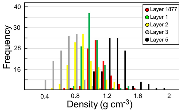
Figure 2. Frequency distributions of bulk density values ( \text{gr cm}^{-3} ) of juvenile fragments for the five selected eruptions (Eruption 1877, and Layers 1, 2, 3, and 5).
