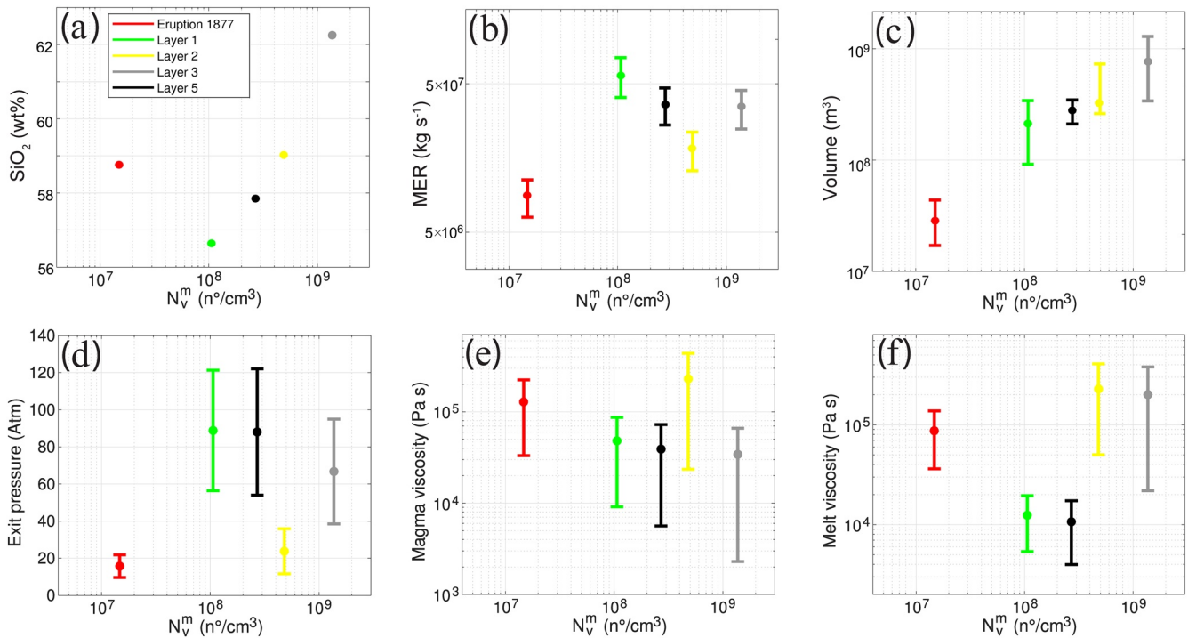
Figure 9. Relationships between Number of vesicles per unit volume ( N_V^m , \text{cm}^{-3} ) of the five selected Cotopaxi eruptions and other key eruption parameters (silica content, mass eruption rate (MER), volume, exit pressure, magma viscosity and melt viscosity) derived from conduit modeling. MER and volume are calculated from the inversion based on Rossi et al. (2019) and Degruyter and Bonadonna (2012) models, and from the average of Exponential, Power Law and Weibull fits, respectively (see Table 1). The variability ranges of the parameters presented in the lower panels were defined considering exclusively the numerical simulations whose results are compatible with textural data (microlites and phenocrysts contents) derived from the studied volcanic products. In other words, we considered the areas enclosed by the red dashed lines in Figures 5–7 and S2–S8 in Supporting Information S1.
