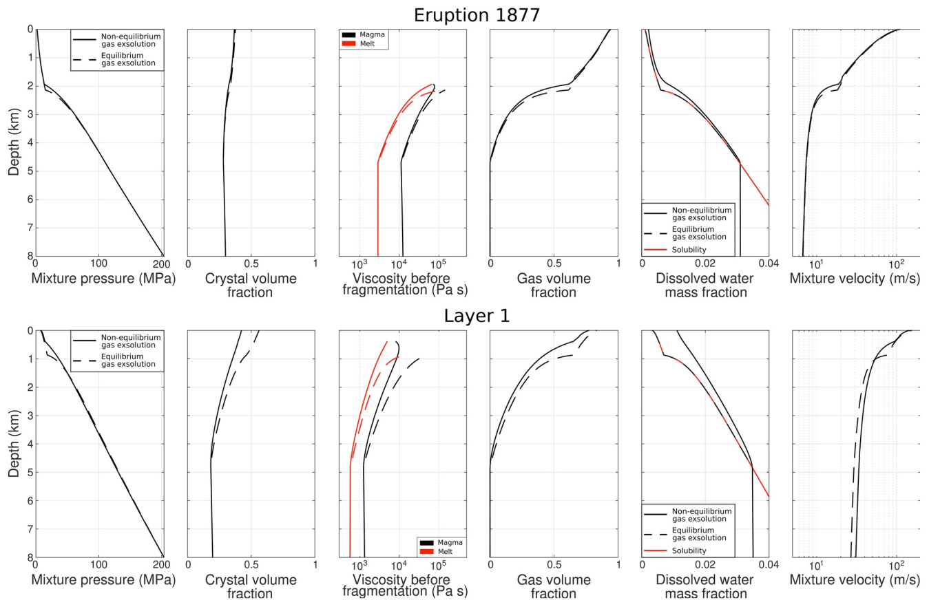
Figure 4. Profiles along the conduit of key physical parameters associated with four specific simulations. Upper panels: Eruption 1877 (equilibrium and non-equilibrium conditions for gas exsolution; water content: 3.1 wt. %; temperature: 950°C). Lower panels: Layer 1 (equilibrium and non-equilibrium conditions for gas exsolution; water content: 3.5 wt. %; temperature: 1000°C). Conduit radius was defined in order to reproduce the computed mass eruption rate of each eruption (Table 1). Other input parameters are presented in Table 3.
