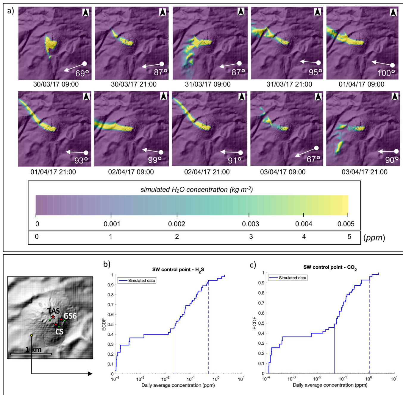
Fig. 8. a) Temporal evolution of the simulated gas dispersion around La Soufrière from 30/03/2017 to 03/04/2017; b) simulated averages of H 2 S and CO 2 concentrations calculated above a control point (643,108 E; 1,774,190 N; yellow dot, Fig. 1d) outside the dome area, along the SW flank of the volcano, from 30/03/2017 to 3/04/2017. The wind field was calculated by using the local meteorological data. The topography is represented by a 5 m resolution DEM. The computational grid has a 15 m resolution.
