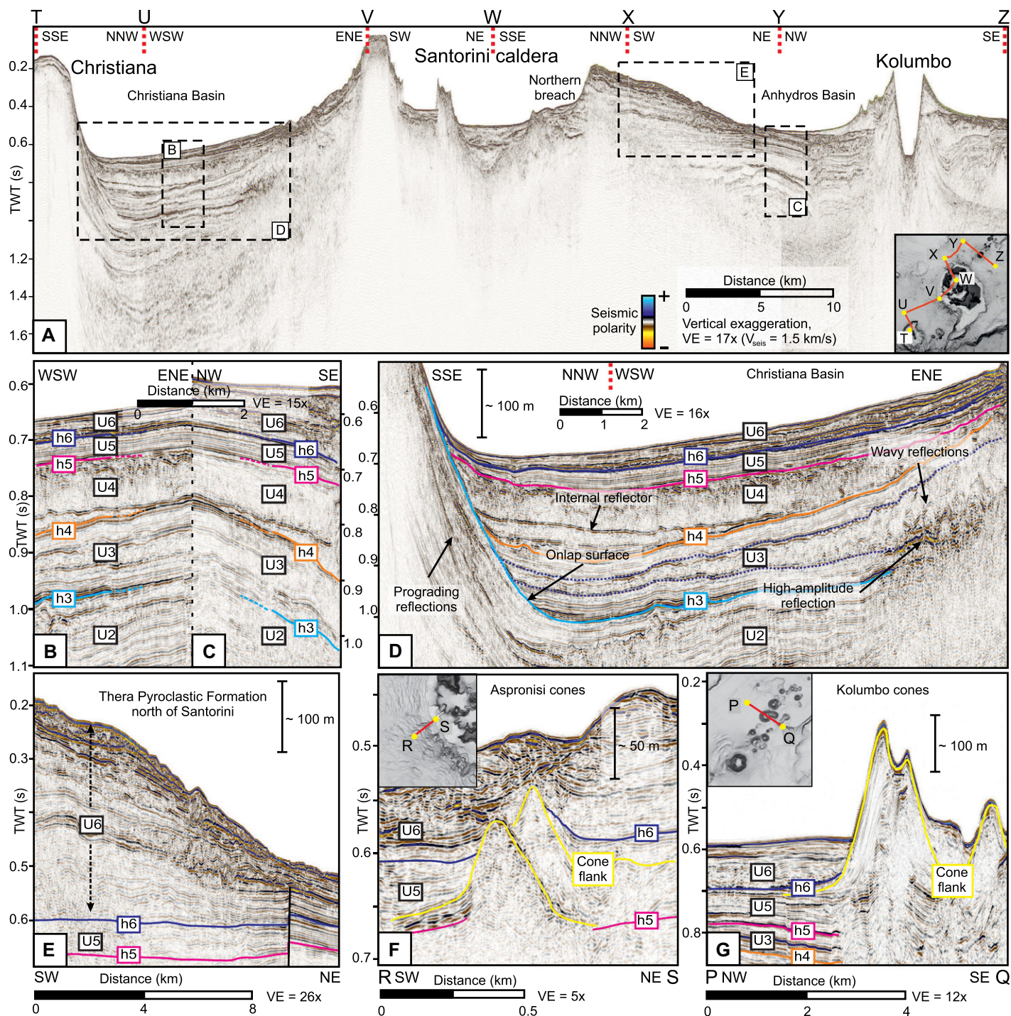
Figure 2. (A) Seismic profile connecting volcanic centers of the Christiania-Santorini-Kolumbo volcanic field. For location, see inset map and Figure 1. (B–E) Enlargements highlight stratigraphic correlation of the upper units of the Christiania (B) and Anhydros Basins (C), the internal architecture of Christiania Basin (D), and the northeastern flank of Santorini (E). (F,G) Additional seismic lines show Aspronisi cones (F) and examples of cones from the Kolumbo chain (G). TWT—two-way travelttime; V_{\text{seis}} —seismic velocity; h3–h6—marker horizons; U2–U6—volcano-sedimentary units.
