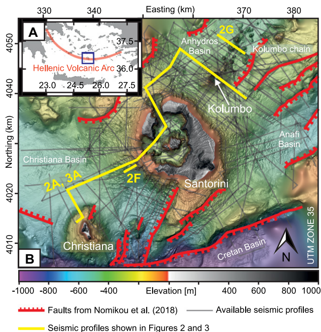
Figure 1. (A) Regional setting of the southern Aegean Sea with study area (blue box). (B) Morphological map of the Christiania-Santorini-Kolumbo volcanic field showing basins, volcanic centers, and volcanic lineaments. UTM—Universal Transverse Mercator.
