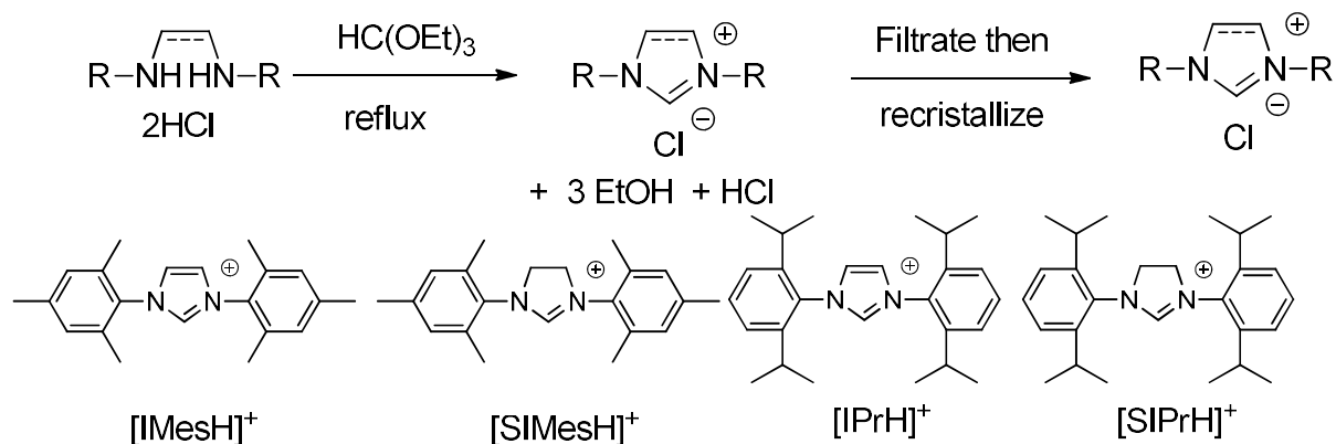
Scheme 1: Imidazolium and imidazolinium synthesis.
