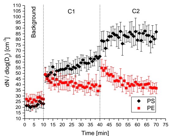
S7: Normalized mean particle size distribution measured by the OPC for PS 350 nm and PEnano with different generated bubble sizes. For clarity purpose, particles concentrations measured with SDS solution only was used as background signal and subtracted from the signal generated following particle addition, an average of 10 min for each being considered.
