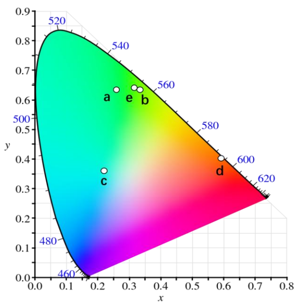
Fig. 9. CIE 1931 chromaticity coordinates of the different silicone/LDH-PAO (40 wt%) films: (a) LDH-AO/C343, (b) LDH-AO/HPTS, (c) LDH-AO/C3C, (d) LDH-AO/RhB and (e) LDH-UV/HPTS.
