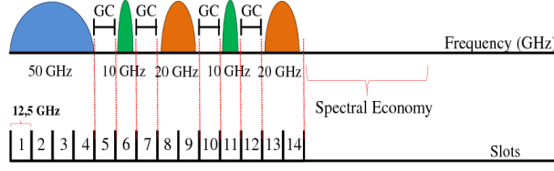
Fig. 1. Slot concept illustration in SFONs [77].
