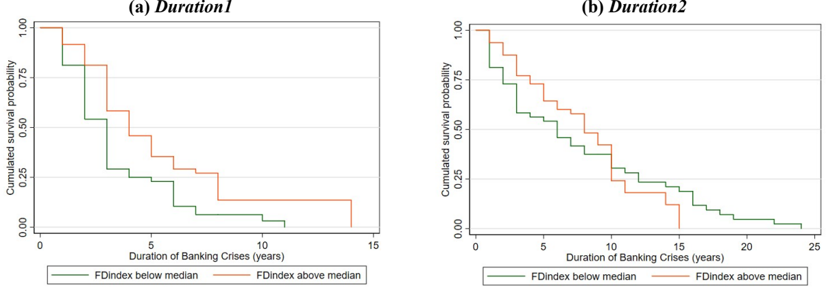
Figure 1. Kaplan-Meier survival functions for the DBC according to FDindex
