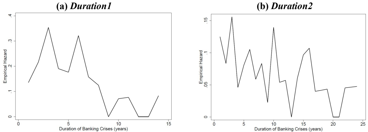
Figure 2. Estimated empirical hazard of DBC
