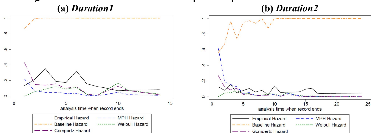
Figure 3. Performance of the MPH compared to parametric duration models
