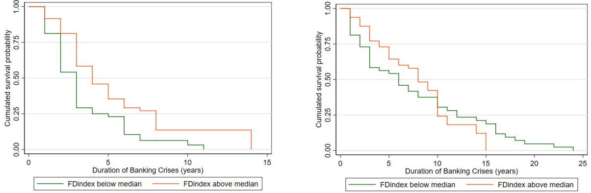
Figure 1. Kaplan-Meier survival functions for the DBC according to FDindex (a) Duration1 (b) Duration2
