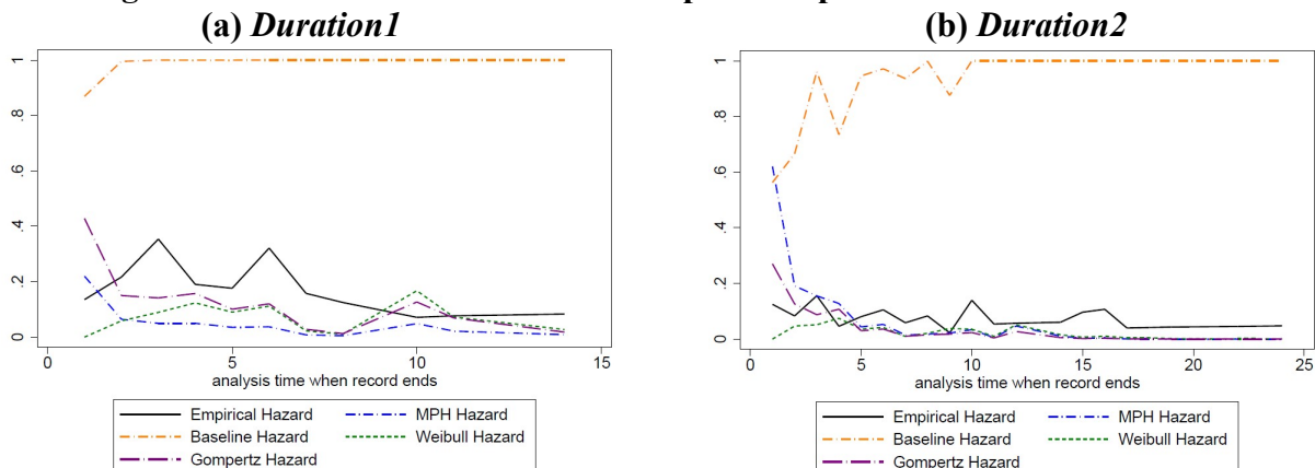
Figure 3. Performance of the MPH compared to parametric duration models
