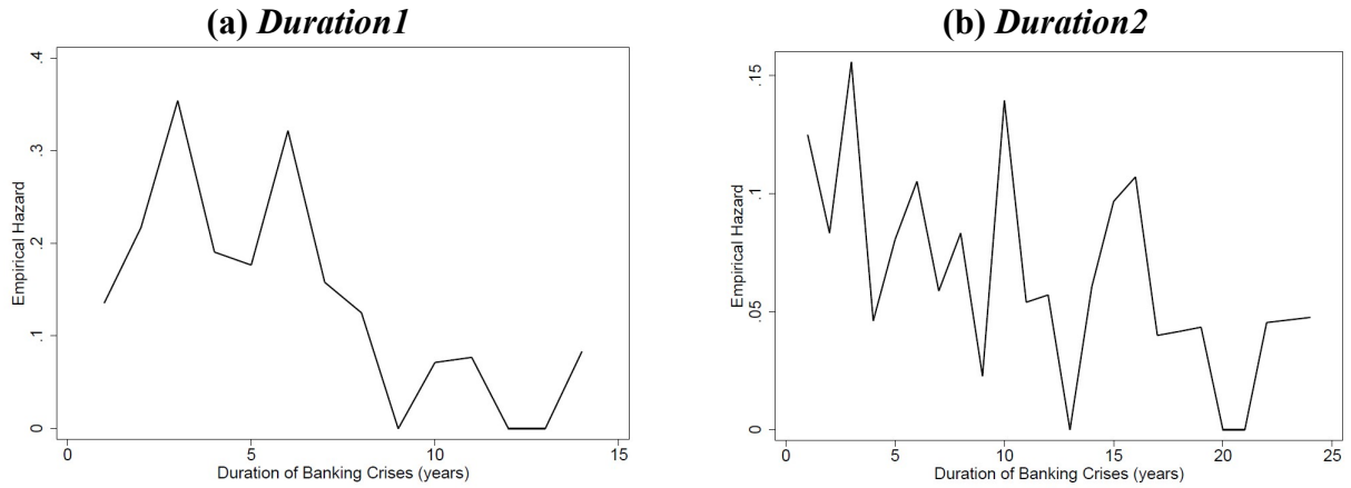
Figure 2. Estimated empirical hazard of DBC
