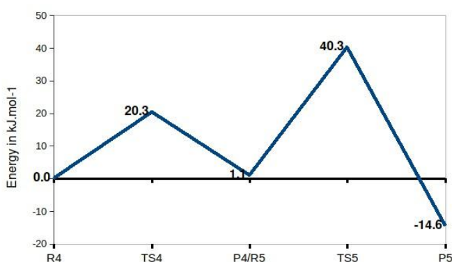
Figure 13. Profile of Free Gibbs energy ( \text{kJ}\cdot\text{mol}^{-1} ) from acyl-enzyme to product stage. R4, TS4 and P4: IRC reactant, TS and IRC product of addition of acyl-enzyme on DR5P step. R5, TS5 and P5: IRC reactant, TS and IRC product of ThDP regeneration and release of DS7P step
