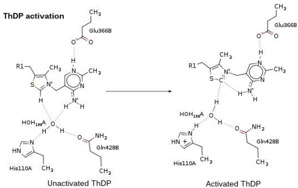
Scheme 1. Overview of ThDP activation
