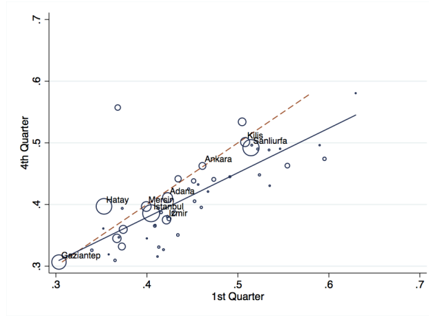
(a) Dissimilarity index D
