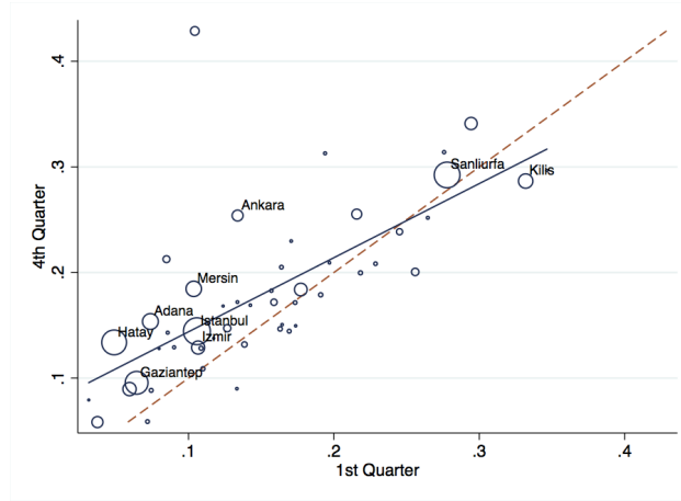
(b) Normalized isolation index I^{\text{adj}}
