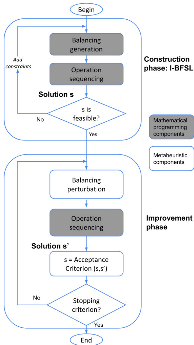
Fig. 4: General scheme of the proposed metaheuristic
