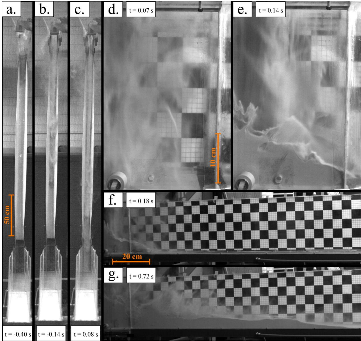
Figure 3. Stages observed in the experiments. a. b. c. Acceleration and dilation of the granular mixture inside the open column upon release from the hopper (experiment 13; Table 1). d. e. Impact of the granular mixture onto the channel base and accumulation of particles (experiment 9; Table 1). f. g. Lateral propagation of the granular flow (experiment 10; Table 1). The time t = 0 s corresponds to the arrival of particles at the impact zone.
