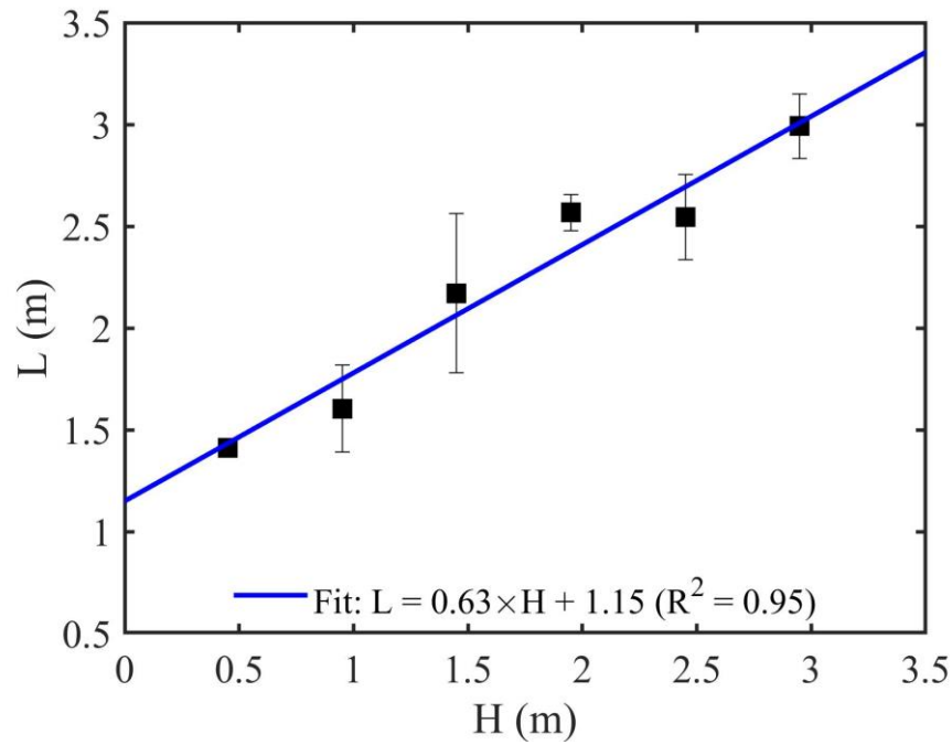
Figure 9. Maximum runout distance L of the flows as a function of the fall height H (solid symbols). The blue line shows the linear best fit of the data. Error bars account for runout variations among the 7 repeats that were possibly caused by particles ejected above the channel walls during flow emplacement and the generation of more vigorous and voluminous spray of particles at impact (i.e. phase 1), respectively.
