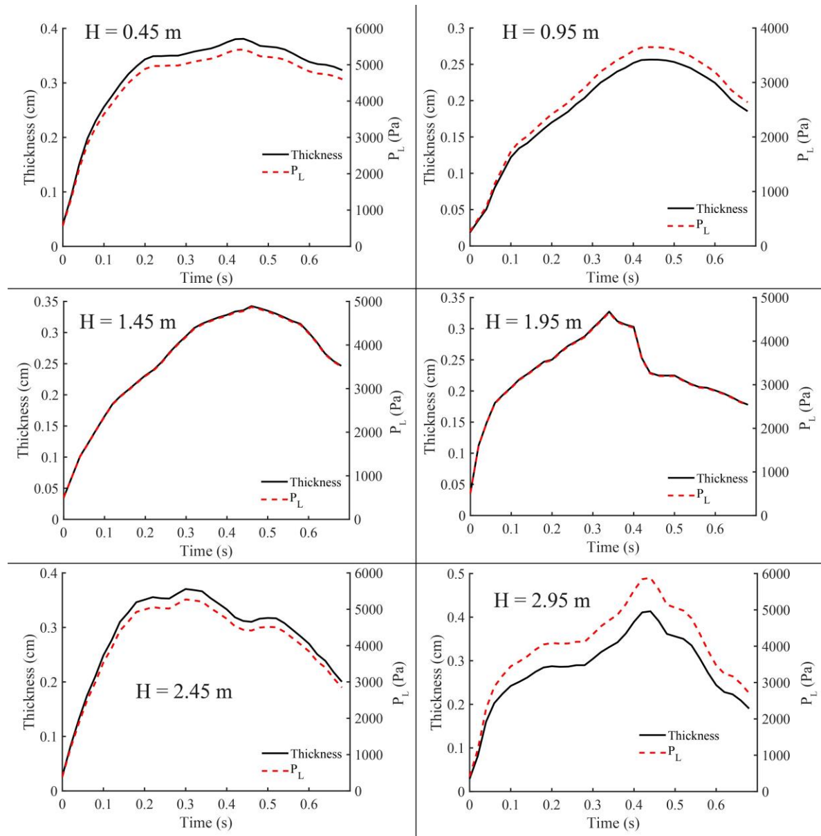
Figure S1. Thickness of the granular material (solid black line) at the impact zone and maximum estimate of the lithostatic pressure for C = 0.46 vol. % (red dashed line P_L ) as a function of time. Results are shown for fall heights H = 0.45 - 2.95 m.
