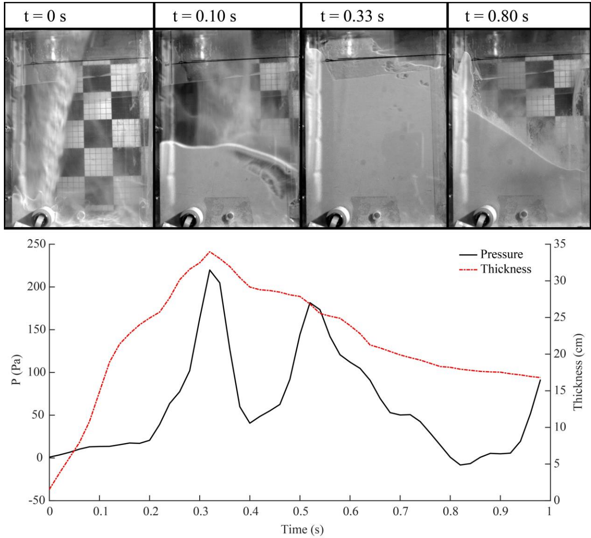
Figure 5. Pore fluid pressure ( P ; solid black line) and thickness of the granular material (dash-dotted red line) as a function of time for experiment 5 ( H = 1.45 m; Table 1). Images of the impact zone are synchronized with the pressure signal and show the accumulation of the granular mixture. We could not investigate the motion of the granular mixture after impact in order to determine the contribution of the dynamic pressure on P .
