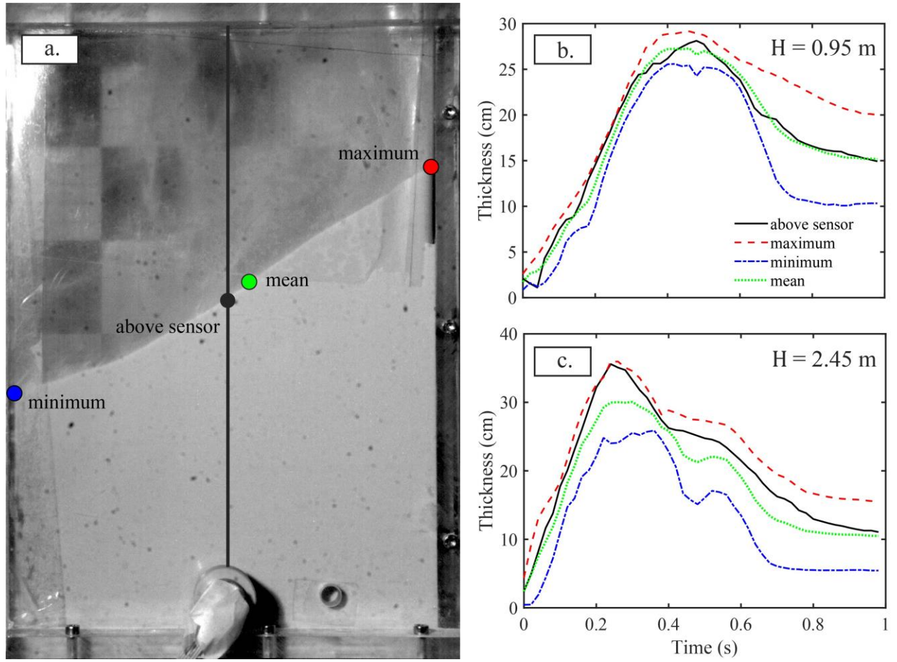
Figure S3. Thickness of the granular material measured at different locations in the impact zone shown in panel (a). (b) Experiment 3, H = 0.95 m. (c) Experiment 9, H = 2.45 m. The granular bed varies significantly in thickness. The lithostatic pressure is calculated considering the bed thickness above the sensor, which is very close to the mean thickness.
