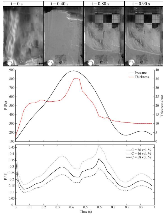
Figure S5. Evolution of P/P_L for experiment 11 ( H = 2.95 m; Table 1), considering different values of the particle concentration in the dense granular bed: C = 36 vol. %, which is the maximum concentration in the column, C = 46 vol. %, typical of a bubbling granular bed, and C = 58 vol. % for a random packing.
