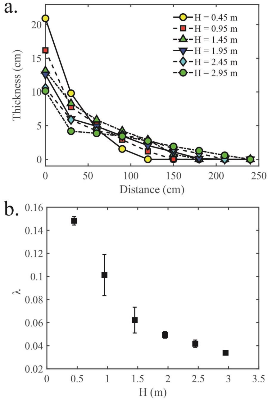
Figure 11. a. Deposit morphology at six different fall heights. b. Deposit aspect ratio \lambda as function of the fall height.
