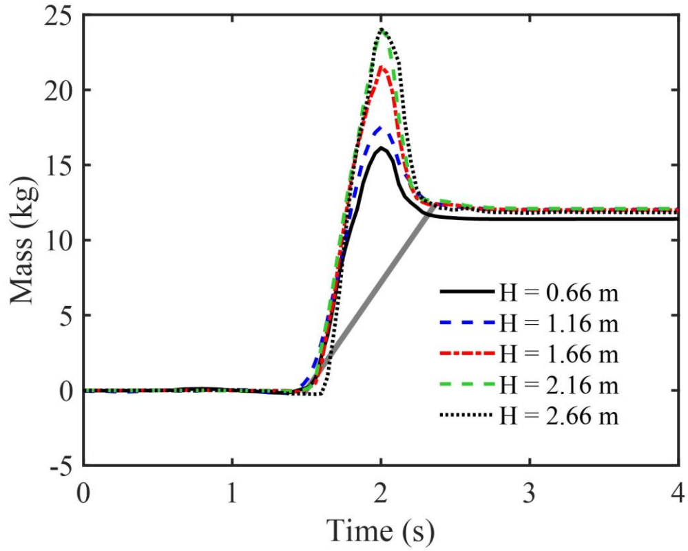
Figure 2. Particle supply from the hopper recorded by the static scale. The mass of particles released is shown as a function of time for five different fall heights, H . Notice that the apparent mass measured is larger than that released (12 kg, recovered after \sim 2.3 s) because of the non-zero velocity of the particles at impact in the container. Therefore, we estimated the time-averaged mass flux from the slope of the solid grey line indicating the time at which the initial mass in the hopper was recovered.
