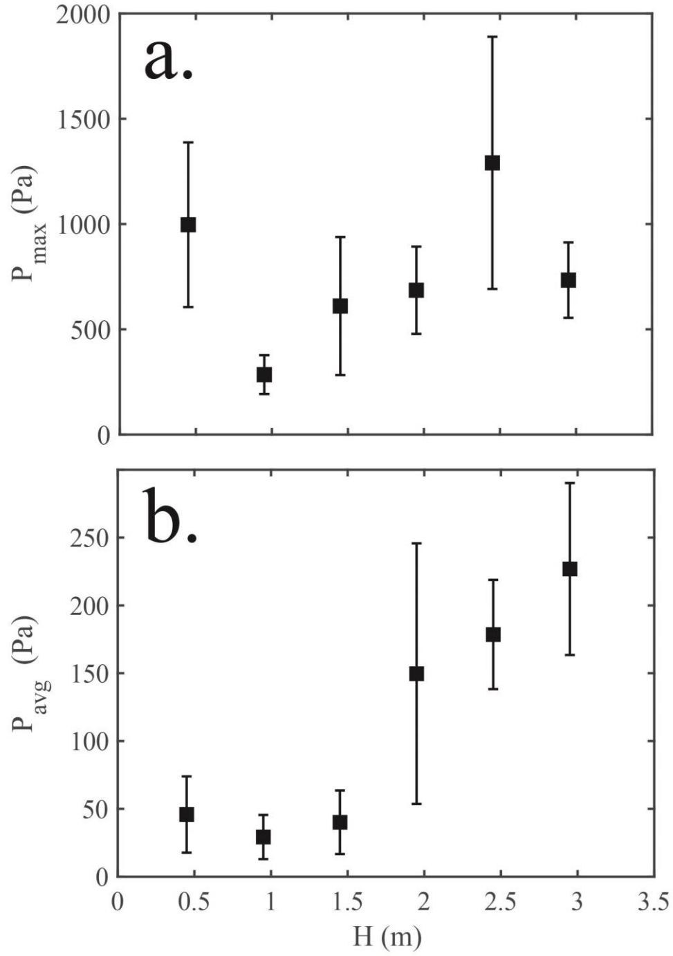
Figure 6. a. Maximum pore fluid pressure P_{\max} measured at impact zone as a function of the fall height, H . b. Average pore fluid pressure P_{\text{avg}} generated in the first second following impact, as a function of H .
