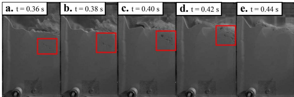
Figure S4. Air bubbles formed during compaction of the granular material at impact zone (experiment 9; Table 1).
