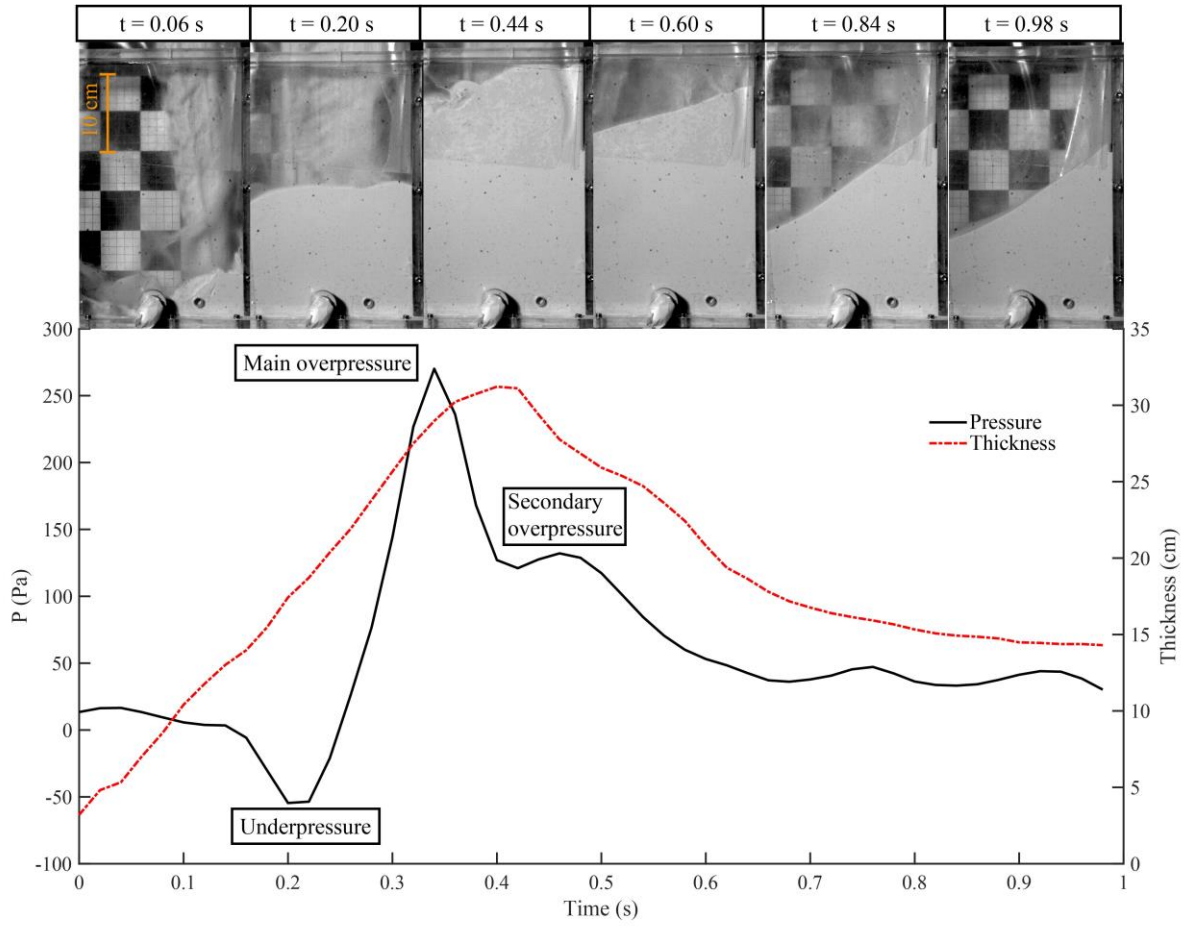
Figure S2. Pore fluid pressure ( P ; solid black line) and thickness of the granular material (dash-dotted red line) as a function of time for an experiment with an initial underpressure phase (experiment 3; H = 0.45 m; Table 1). Images of the impact zone are synchronized with the pressure signal and show the accumulation of the granular mixture.
