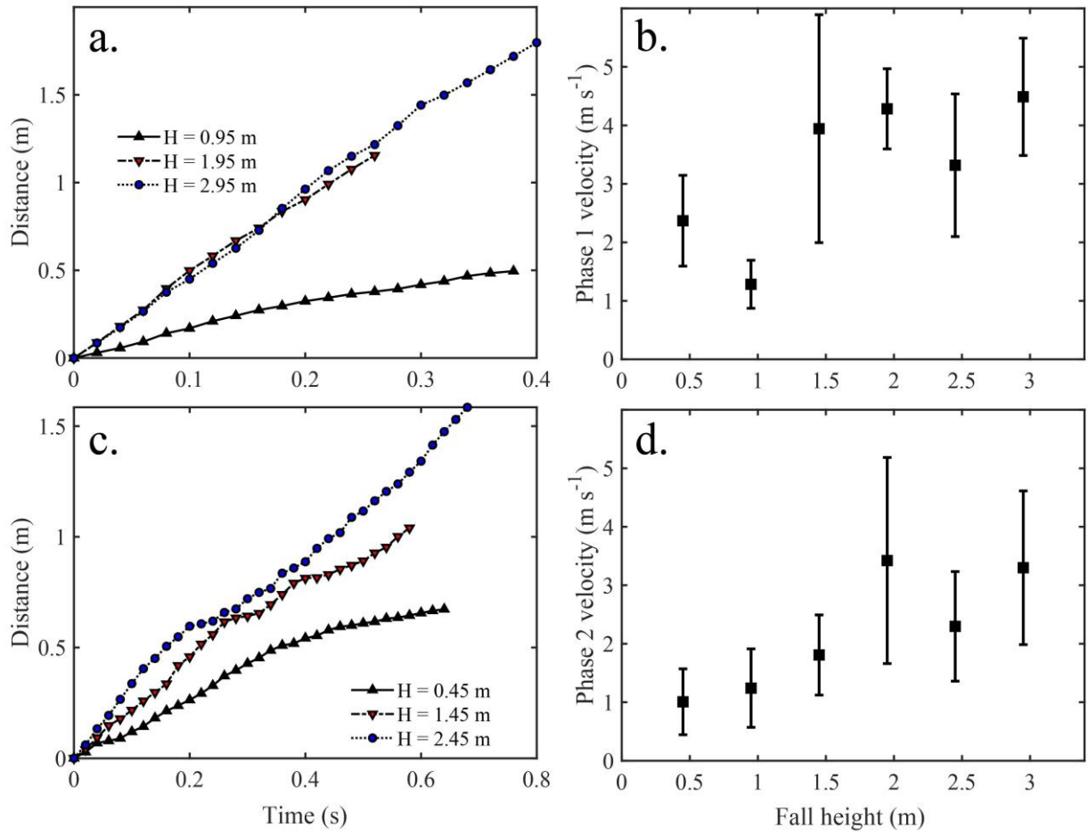
Figure 10. Flow kinematics and mean front velocity as a function of the fall height during phase 1 (a., b.) and phase 2 (c., d.). Note that phase 1 flow is out of the video frame after 0.28 s for H = 1.95 m and that no data were collected after that time.
