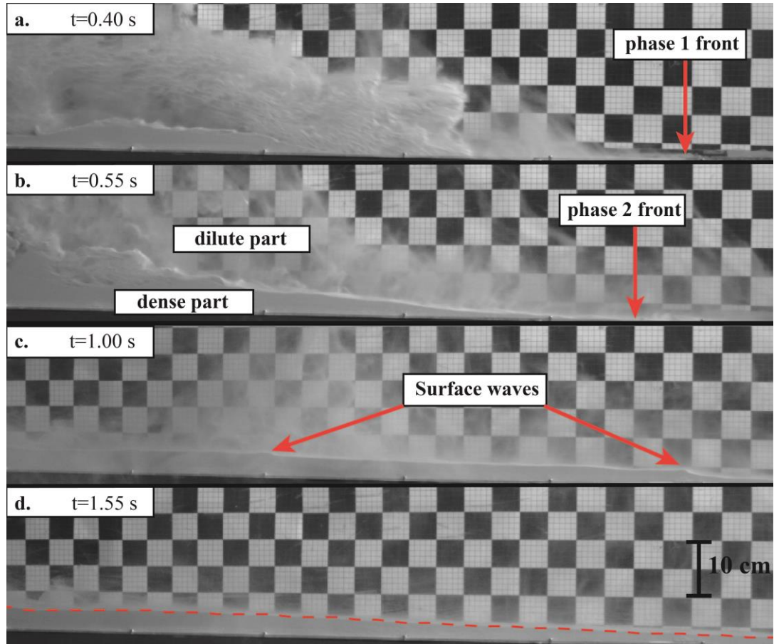
Figure 8. Flow emplacement in the channel at (a) t = 0.40 s, (b) t = 0.55 s, (c) t = 1.00 s, and (d) t = 1.55 s during experiment 12 ( H = 2.95 m; Table 1). Panels a, b, and c correspond to phases 1 (fast-moving thin flow), 2 (slower pulsatory dense flow) and 3 (thickening of the deposit), respectively. Panel d shows the final deposit.
