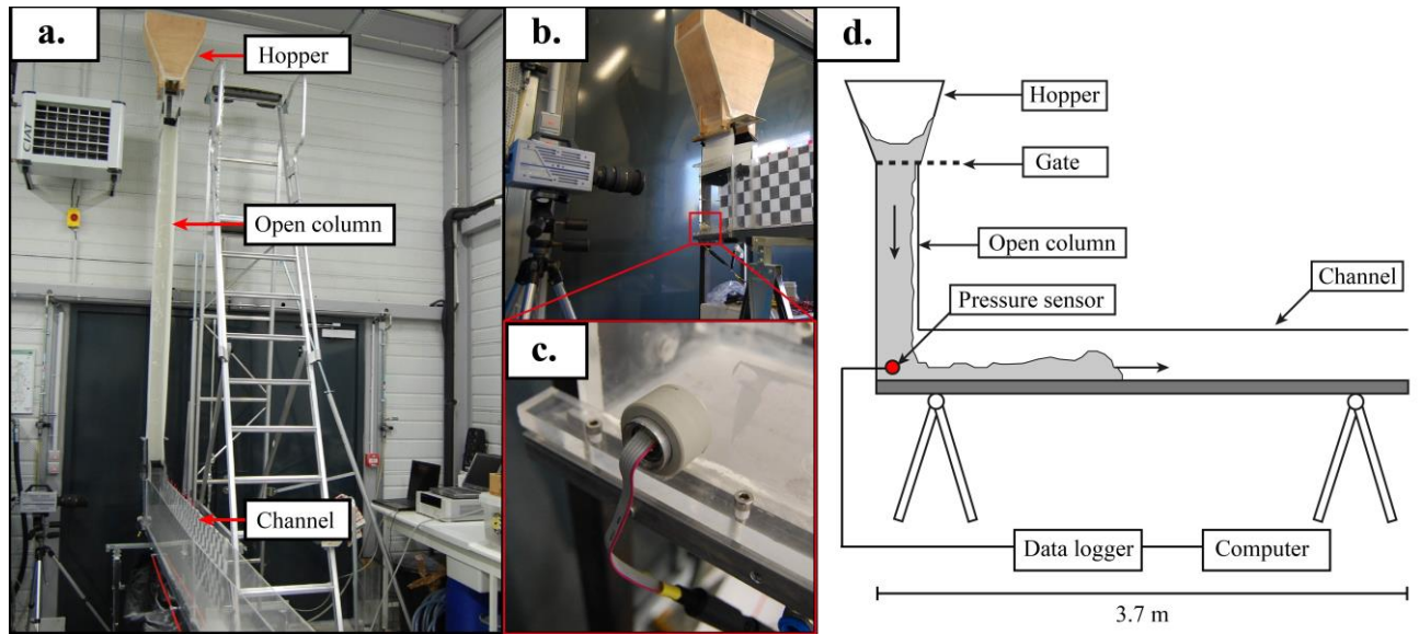
Figure 1. Experimental apparatus. (a) Longitudinal view with the hopper in the highest position. (b) Hopper in the lowest position and high-speed camera set to monitor the impact zone. (c) Pressure sensor at the sidewall of the impact zone. (d) Sketch of the experimental set-up.
