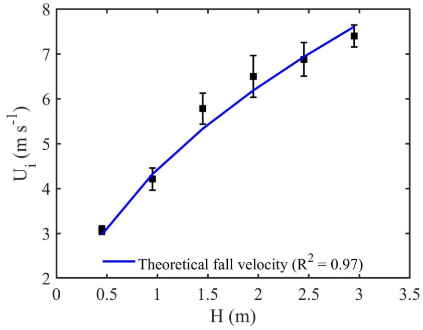
Figure 4. Fall velocity of the particles at the impact zone as a function of fall height H (solid symbols). The blue curve represents the predicted free fall velocity using U_i = \sqrt{2gH} .
