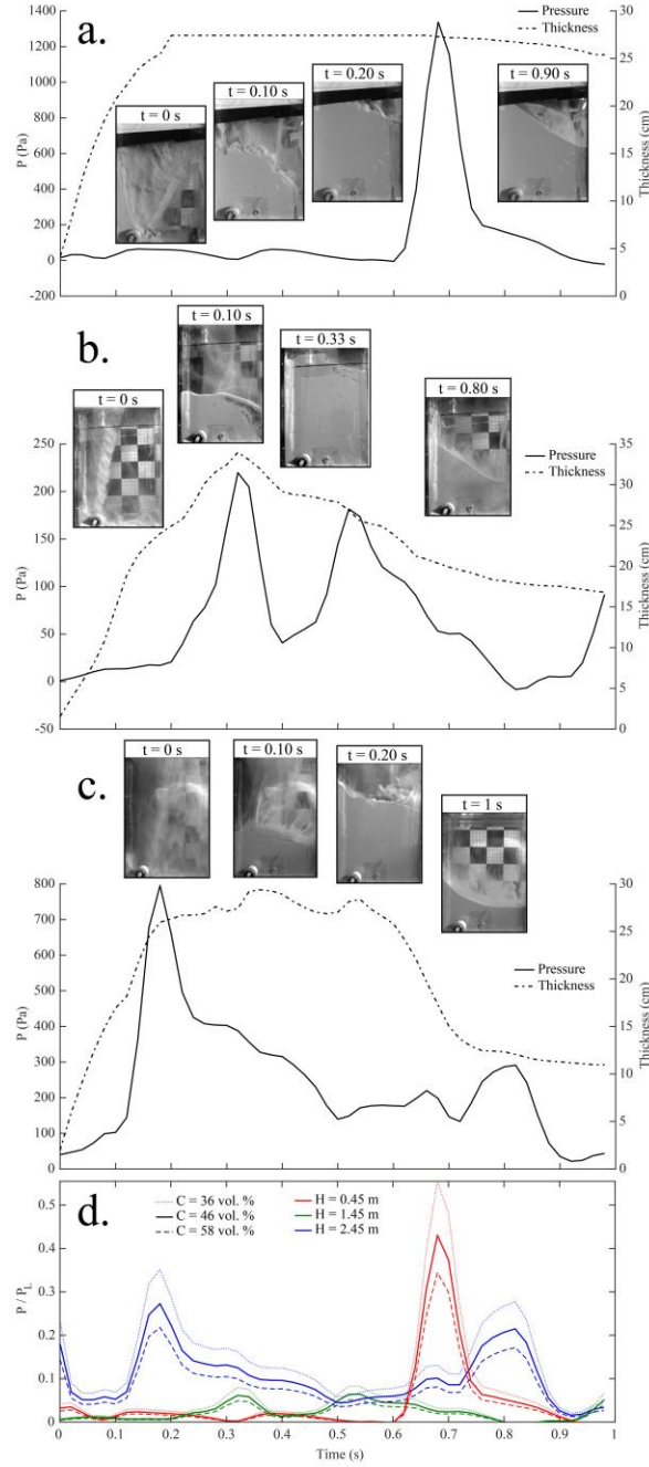
Figure 7. Pore fluid pressure and thickness of the granular bed measured at impact zone as function of time for a. experiment 1 ( H = 0.45 m; Table 1), b. experiment 5 ( H = 1.45 m; Table 1), and c. experiment 9 ( H = 2.45 m; Table 1). d. Ratio P/P_L of the pore fluid pressure over the lithostatic pressure of the granular bed as a function of time for the experiments presented above, assuming different particle concentrations. The minimum bed concentration C = 36 vol. % corresponds to the maximum concentration of the falling mixture, and the maximum concentration C = 58 vol. % is that of a loosely packed bed. Higher resolution images of the impact zone are provided in Figure S6.
