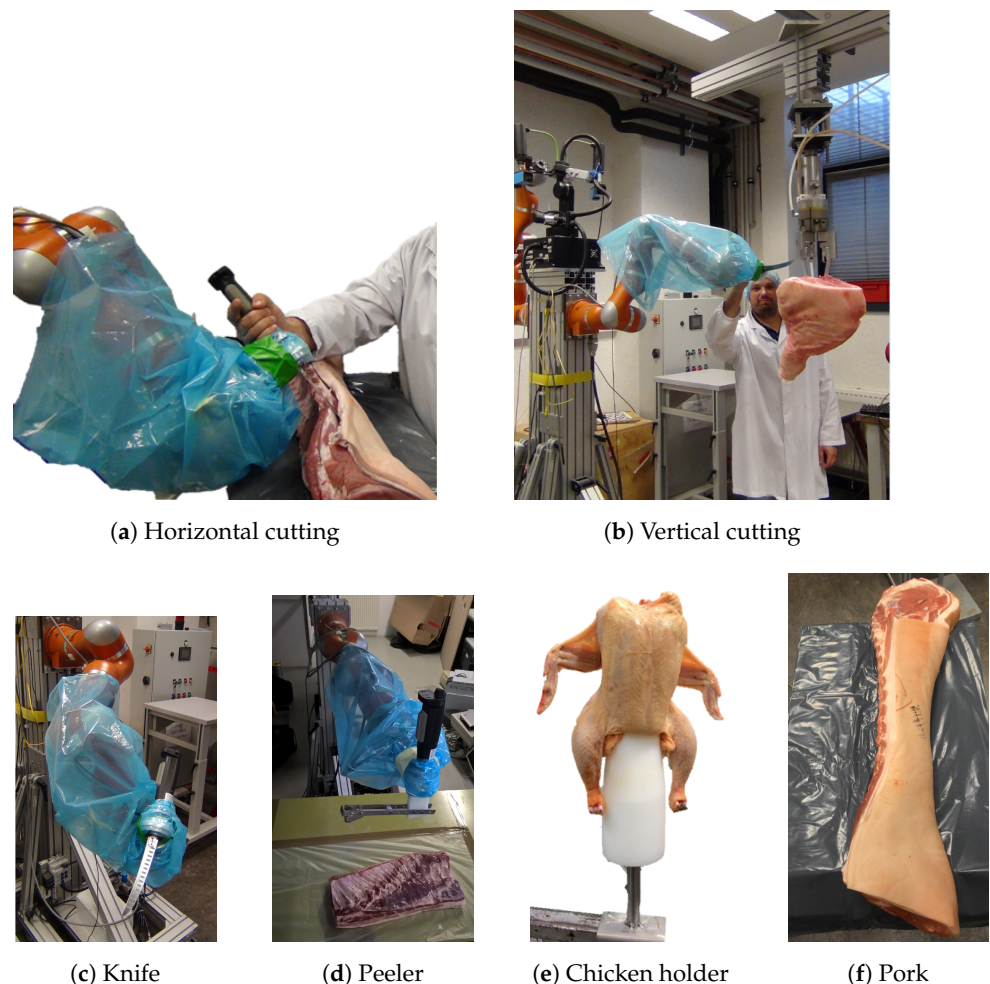
Figure 13. Exoscarne equipment.
