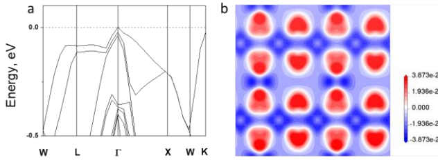
Figure 8: Magnified/zoomed representation of the top of the valence band of \gamma - \text{Ge}_3\text{N}_4 confirming direct nature of band gap (a) and electron density difference in cross-section oriented along (0, \sqrt{2}/2, \sqrt{2}/2) direction and half bond shifted (in electrons/ \text{\AA}^3 ).
