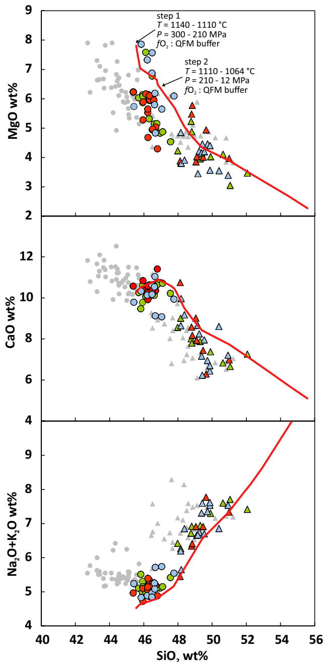
FIGURE 4 Major element compositions in restored melt inclusions (MIs) after correction for \text{SiO}_2\text{-H}_2\text{O} loss. Unrestored MIs are reported for comparison (symbols as in Figure 3). Results from rhyolite-MELTS simulations on restored MIs (red line) and parameters used for each step of simulation are reported
