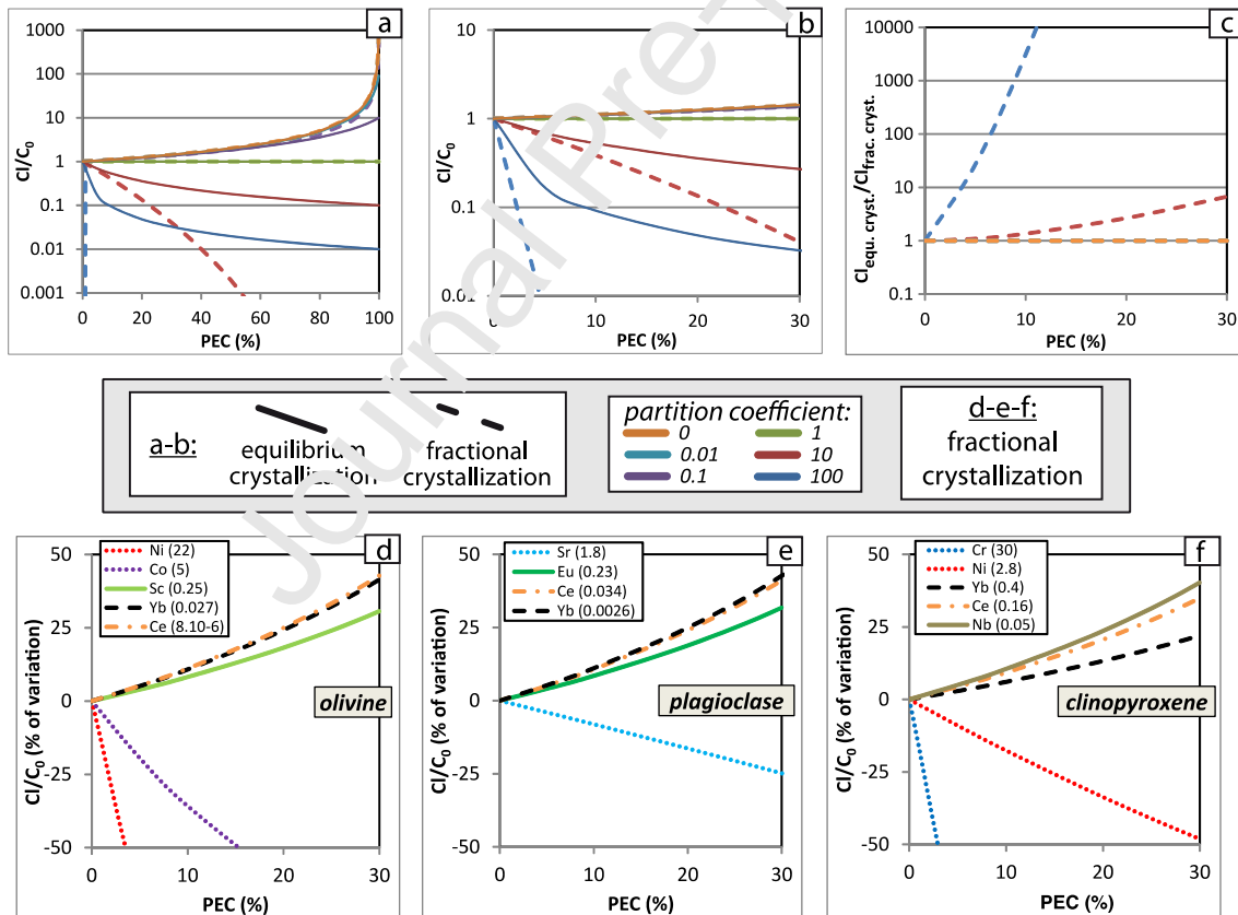
Fig. 10: Evolution of trace elements contents during PEC. a-b) present the evolution of the melt inclusion content (Cl) relative to initial content (C 0 ) for elements with various partition coefficients. In c-e) the variation is presented in percent of variation relative to
