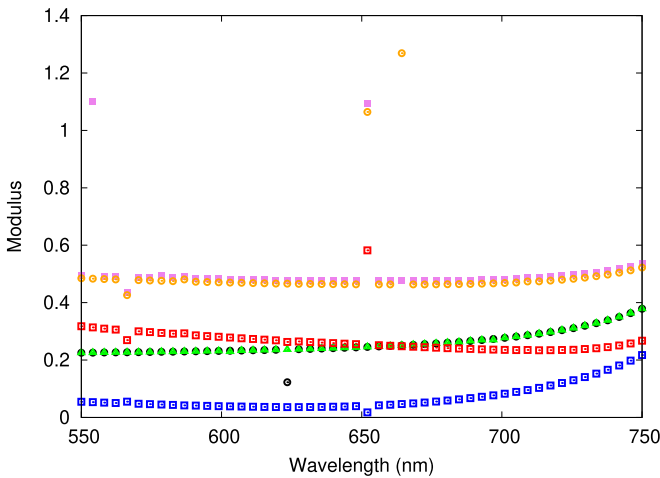
FIG. 11. Coefficient reflection for the Bloch mode depending on the simple Bragg mirror (i) beginning with a high index layer (green triangles), (ii) beginning with a low index layer (black circles), (iii) beginning with adapted layers on the air side (blue squares), (iv) terminating with adapted layers on the silicon side (red squares), (v) terminating with a high index layer (pink squares), or (vi) terminating with a low index layer (orange circles). Clearly the adapted layers reduce the reflection for the Bloch mode.
