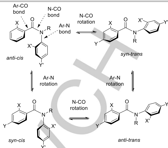
Figure 5. Different conformations accessible by rotation about the Ar–N, Ar–CO and N–CO bonds
