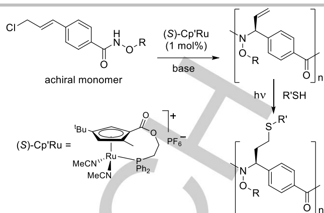
Scheme 3. Asymmetric polymerisation to access optically active poly- N -alkoxyamides.
