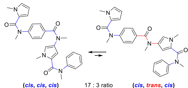
Scheme 11. Proportion of conformers observed by NMR in \text{CD}_2\text{Cl}_2 at 233K.
