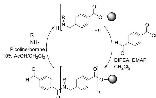
Scheme 9. Submonomer synthesis of aryloptoids using an alternative acylation – reductive amination cycle.
