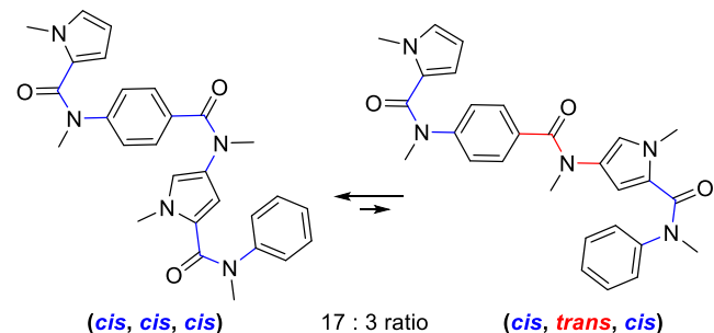
Scheme 11. Proportion of conformers observed by NMR in CD 2 Cl 2 at 233K.
