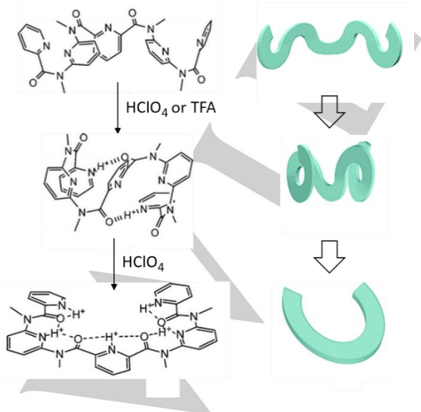
Scheme 12. Acid-responsive conformations of an N -methyl aromatic oligoamide made from 2,6-disubstituted pyridines (adapted from reference [17c] with permission from American Chemical Society).
