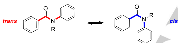
Figure 3. Cis/trans isomerism of N -alkylated aryl amides.
