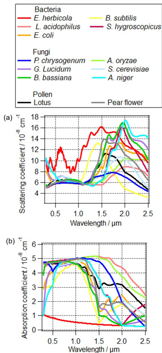
Figure 6. The influence of different PBAPs on (a) the scattering coefficient and (b) absorption coefficient of total particles. The refractive indices are based on the measurements by Arakawa et al. (2003) and Hu et al. (2019).
