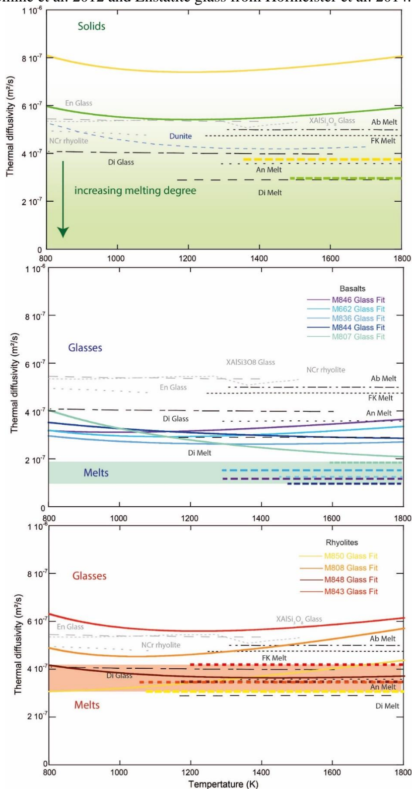
Figure 8: Comparison with the literature of our thermal diffusivities obtained our peridotite (upper panel), basaltic (center panel) and rhyolitic (lower panel) starting materials. Solids (peridotite and glasses) and melts are represented in thick lines and thick dashed line, respectively. Literature data are reported with thinner dashed lines (grey to black). Diopside (Di) glass and melt, XAlSi 3 O 8 glass, Anorthite melt (An), Albite melt (Ab) and orthose melt (FK) from Hofmeister et al. 2009, NCr Rhyolite from Romine et al. 2012 and Enstatite glass from Hofmeister et al. 2014.
