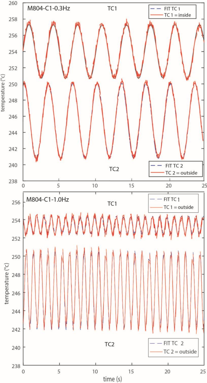
1220 Figure 3: Examples of temperature waves recorded at high temperature during M804 experiments. 1221 Such data set is acquired after the sample equilibration at target temperature conditions for a few 1222 minutes (here T = 250^{\circ}\text{C} ). Acquisitions are performed at an interval ranging from 40 ms to 200 ms. 1223 At least 10 periods of the temperature oscillation are recorded to ensure a good extraction of phase 1224 shifts and amplitude ratio based on the fitting procedure described in Methods. Upper and lower 1225 frames correspond to temperature measurements performed at frequencies of 0.3 and 1 Hz, 1226 respectively. Red symbols are measured data and the dash thick lines represent the fitted sine waves. 1227
