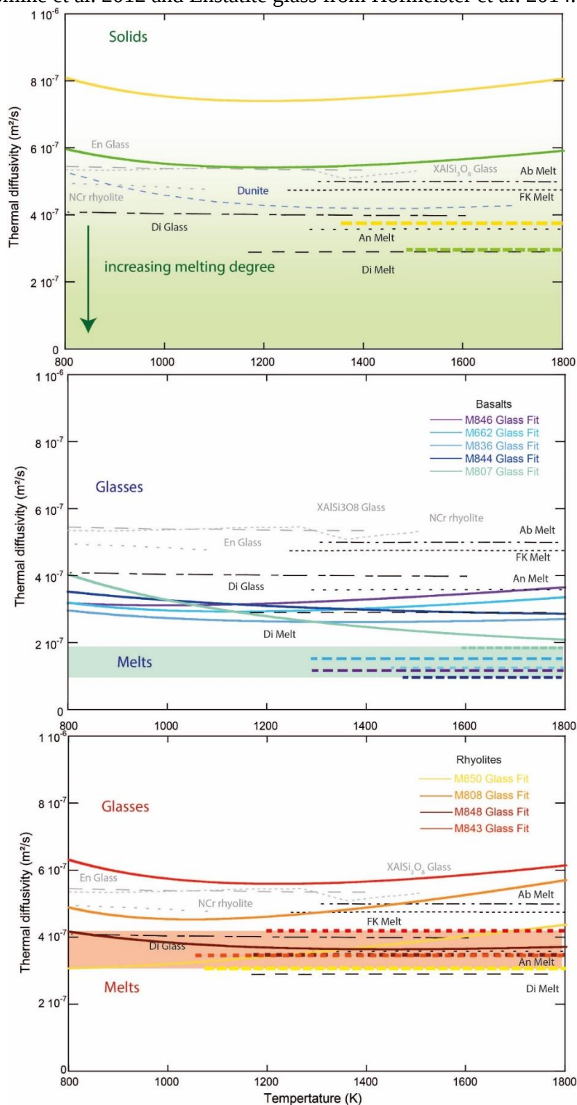
1262 Figure 8: Comparison with the literature of our thermal diffusivities obtained our peridotite (upper 1263 panel), basaltic (center panel) and rhyolitic (lower panel) starting materials. Solids (peridotite and 1264 glasses) and melts are represented in thick lines and thick dashed line, respectively. Literature data 1265 are reported with thinner dashed lines (grey to black). Diopside (Di) glass and melt, \text{XAlSi}_3\text{O}_8 glass, 1266 Anorthite melt (An), Albite melt (Ab) and orthose melt (FK) from Hofmeister et al. 2009, NCr 1267 Rhyolite from Romine et al. 2012 and Enstatite glass from Hofmeister et al. 2014.
