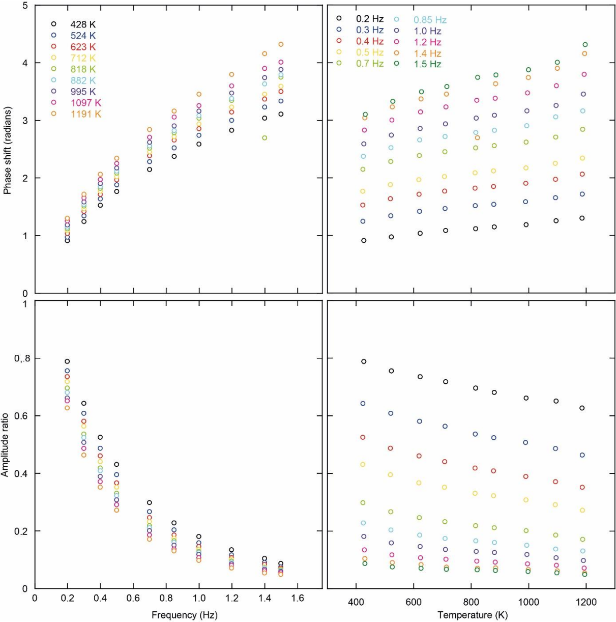
1230 Figure 4: Example of refined phase shifts (top panels) and amplitude ratio (bottom panels) as a 1231 function of frequency (from 0.2 to 1.5 Hz, left panels) and temperature (from 428 K to 1191 K, right 1232 panels) for sample M844. 1233
