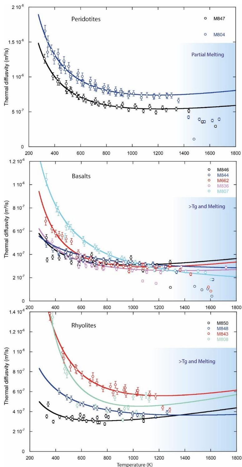
1248 Figure 6: Thermal diffusivities data refined for our peridotites, basalts and rhyolites samples (from 1249 top to bottom) as a function of temperature. Associated fits are represented with a solid line of the 1250 same color than the symbols. Error bars are shown when larger than the symbol size. Several basaltic 1251 (M807, M662) and rhyolite (M848, M808) samples were partially recrystallized during the annealing 1252 and dehydration procedures prior to the conductivity measurement, as indicated by their high 1253 conductivity values at low temperatures. Thermal diffusivities values converge at high temperatures 1254 and melting.
