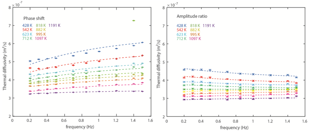
Figure 5: Typical example of a set of raw values of the thermal diffusivity extracted from our measurements for a basaltic glass, presented as a function of the frequency of the heat source. Experimental temperatures range between ~430 and ~1200 K at a pressure of 2GPa (sample M844). Left and right panels correspond to thermal diffusivities calculated from phase shifts and amplitude ratios, respectively. The color code is kept similar in both panels. The fit through the data is made following the equation D = D_0 + A \exp(-f/f_0) (Xu et al., 2004), where D_0 is the high-frequency asymptote of the diffusivity (see text). Error bars are generally within the size of the symbol.
