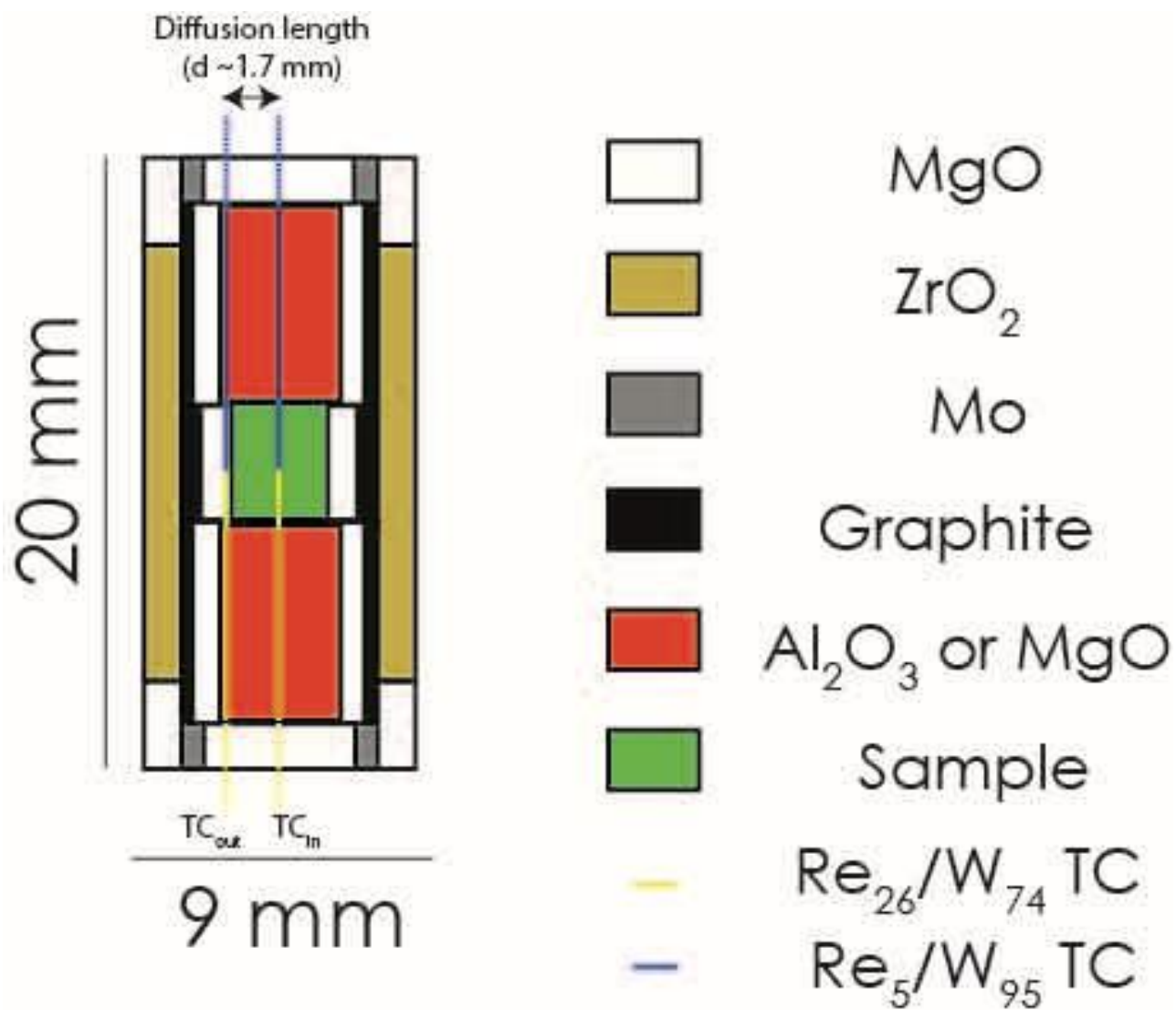
1192 Figure 1: Schematic cross-section of the high-pressure cell assembly used for Angstrom method with 1193 multi-anvil apparatus. For glass and melt experiments, thermocouples were inserted in alumina tubes 1194 of 0.6 mm diameter and 4.5 mm length in the sample zone. 1195
