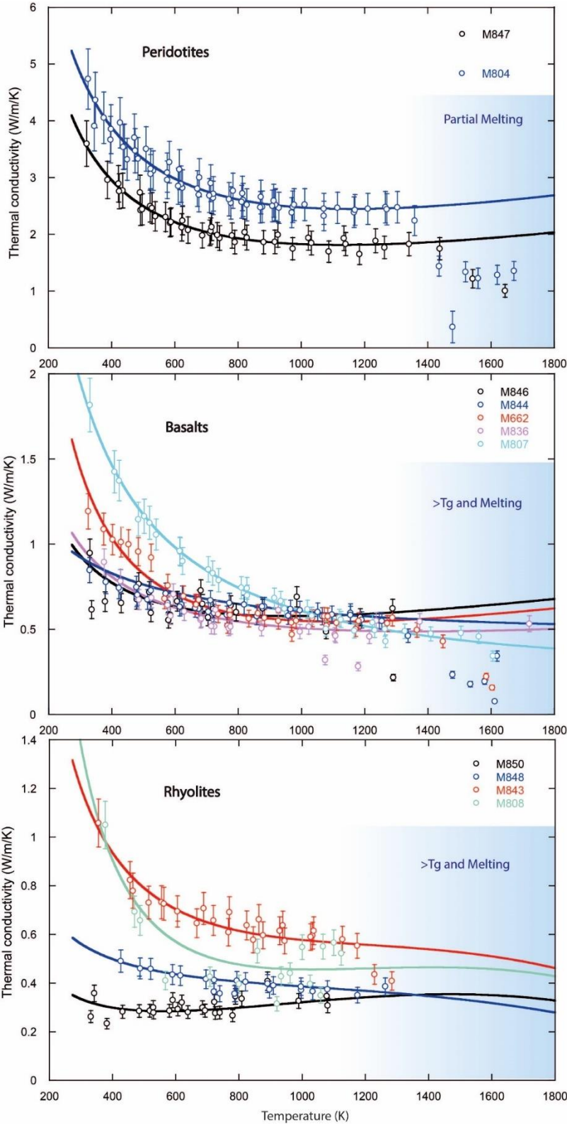
1257 Figure 7: Thermal conductivities inferred from diffusivities (Figure 6), heat capacities and densities 1258 (see Figure S4), based on Eq. 17 of the main text. 1259
