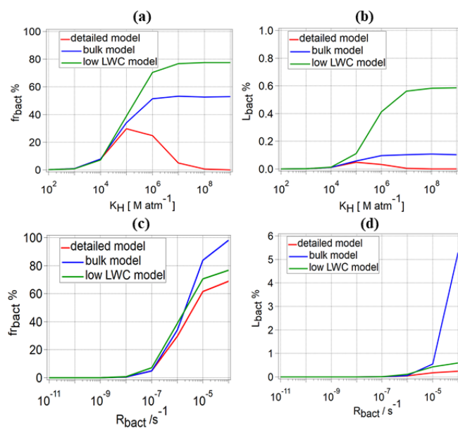
Figure 9. Comparison of (a) fr_{\text{bact}} and (b) L_{\text{bact}} for water-soluble organic gases for three different model approaches: detailed model (red line), bulk approach (blue line), and low-LWC model (green line) for different values of K_H , R_{\text{chemaq}} = 10^{-7} \text{ s}^{-1} , R_{\text{bact}} = 10^{-6} \text{ s}^{-1} , and R_{\text{chemgas}} = 10^{-6} \text{ s}^{-1} ; (c) fr_{\text{bact}} and (d) L_{\text{bact}} for water-soluble organic gases for the same approaches for different R_{\text{bact}} , one value for K_H = 10^5 \text{ Matm}^{-1} , two values for R_{\text{chemaq}} ( 10^{-7} \text{ s}^{-1} , 10^{-11} \text{ s}^{-1} ), and R_{\text{chemgas}} = 10^{-6} \text{ s}^{-1} .
