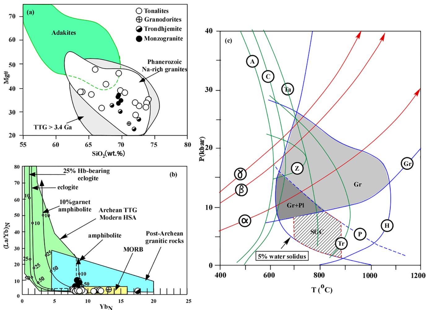
Fig. 16. (a) Mg# vs. SiO 2 variation diagram composed of the SGC with the compositional field of Phanerozoic Na-rich granitoid rocks, >3.4 Ga TTG and Cenozoic adakites. All fields are after Smithies (2000). (b) Chondrite-normalized (La/Yb) N versus Yb N diagram, modified after Jahn et al. (1981) and Martin (1986) showing the compositions of the granitoid phases within the SGC relative to the Archean trondhjemite-tonalite-granodiorite (TTG) field, post-Archean granitic rocks and the range of MORB values. Four partial melting curves are displayed two of which represent melting of amphibolite and 10% garnet amphibolite assuming a MORB source having Yb N = 10 and (La/Yb) N = 1, and the other two represent melting of eclogite and 25% hornblende eclogite, assuming a MORB source with Yb N = 12 and (La/Yb) N = 1 (after Drummond & Defant, 1990). Percent of partial melt values are listed on each of the model curves. (c) Pressure-temperature (P-T) diagram (after Martin & Moyen, 2002) showing the dehydration melting curves of the possible hydrous phases within oceanic crust as well as the geothermal gradients at various times and the stability fields of plagioclase and garnet. In the Early Archean (4.0 Ga), the geothermal gradient (α) was high and any subducted slab melted at shallow depth with plagioclase as a residual phase. At 2.5 Ga, the Earth was cooler and the geothermal gradient (β) was lower and slab melting occurred at greater depth without residual plagioclase. Overlying mantle wedge was thick and hot, and interactions may have occurred between slab melts and mantle peridotite. Geothermal gradient (γ) refers to modern adakites. P-T diagram shows solidus of tholeiite with 5% water as well as main dehydration reactions of oceanic lithosphere. H is hornblende out, A is anthophyllite out, C is chlorite out, Ta is talc out, Tr is tremolite out, Z is zoisite out. G and P outline stability fields of garnet and plagioclase, respectively. Grey field is P-T domain where slab melts can coexist with hornblende- and garnet-bearing residue. Striped area marked SGC represents the possible P-T melting conditions for melts forming the SGC; the melting temperatures are estimated from zircon saturation geothermometry (T zr °C) whereas the upper and lower melting pressure as inferred from the absence of garnet and the presence of residual amphibole in the melting source, respectively.
