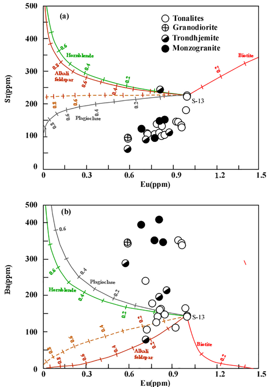
Fig. 14. Sr and Ba vs Eu variation diagrams comparing the Shaitian gneissose granites with liquid lines of descents calculated via Rayleigh fractionation from the least siliceous sample S-13 as a starting composition. Mineral vectors calculated for biotite, plagioclase and alkali feldspar are according to partition coefficients of Bea et al. (1994), whereas mineral vectors calculated for hornblende are based on partition coefficients of Klein, Stosch, and Seck (1997). The dashed lines represent the liquid line of descent if the fractionated assemblage consists of 50% plagioclase and 50% alkali feldspar. Tick marks represent 10% increments of the fractionating mineral.
