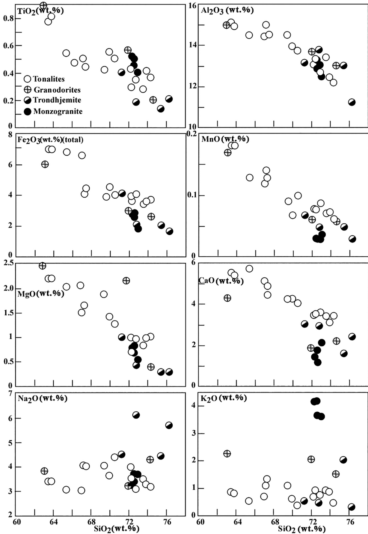
Fig. 4. Bivariate diagrams showing the variation of the measured major elements versus \text{SiO}_2 within the SGC. Mafic xenolith samples exhibit low silica content (<44 wt%) and are omitted from plots for simplicity.
