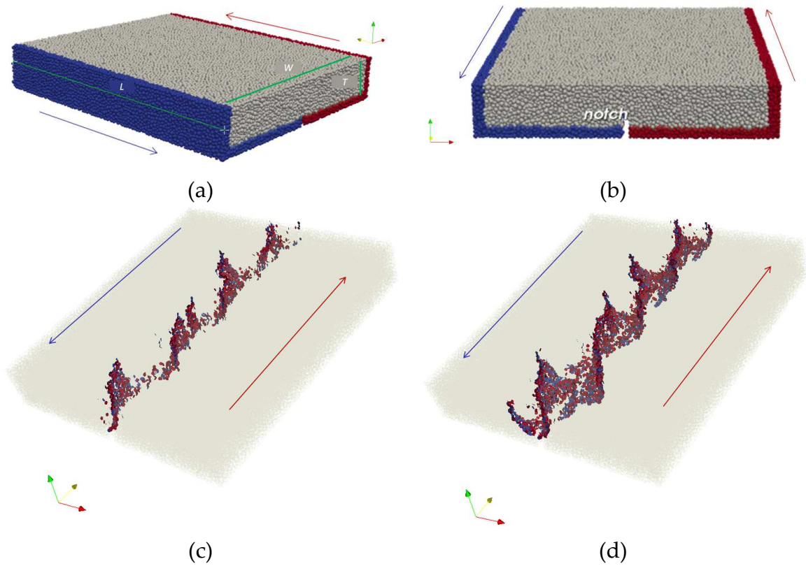
Figure 4. Set up of the numerical model, used to simulate the propagation of en-echelon fractures from a basal parent fault in an elastic brittle layer with x, y, z axes in red, yellow and green color respectively; (a) The perspective view shows the boundary conditions imposed to the model. Colored discrete elements are subjected to an imposed displacement along the fault direction to simulate the shearing process: red discrete elements move in the opposite direction to the blue ones (along the yellow axis y ); (b) Face view showing the presence of the notch at the basement; (c,d) The perspective views show the evolution of the fractures' propagation. Red and blue dots represent local cracks due to mode I and mode II failures respectively, at two different deformation stages.
