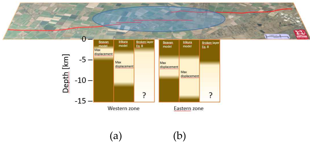
Figure 10. Western (a) and Eastern (b) zones of the Greendale fault represented in Figure 9 . For (a) and (b) respectively, the first column represents the maximum displacement zone according to Beavan et al. (2012) and Irikura et al. (2019) in the second column. In the third column, the dark zone represents the fractured brittle layer above the parent fault at depth (clear zone). The question mark illustrates the fact that Equation 8 can only provide the thickness of the fractured layer above the parent fault at depth.
