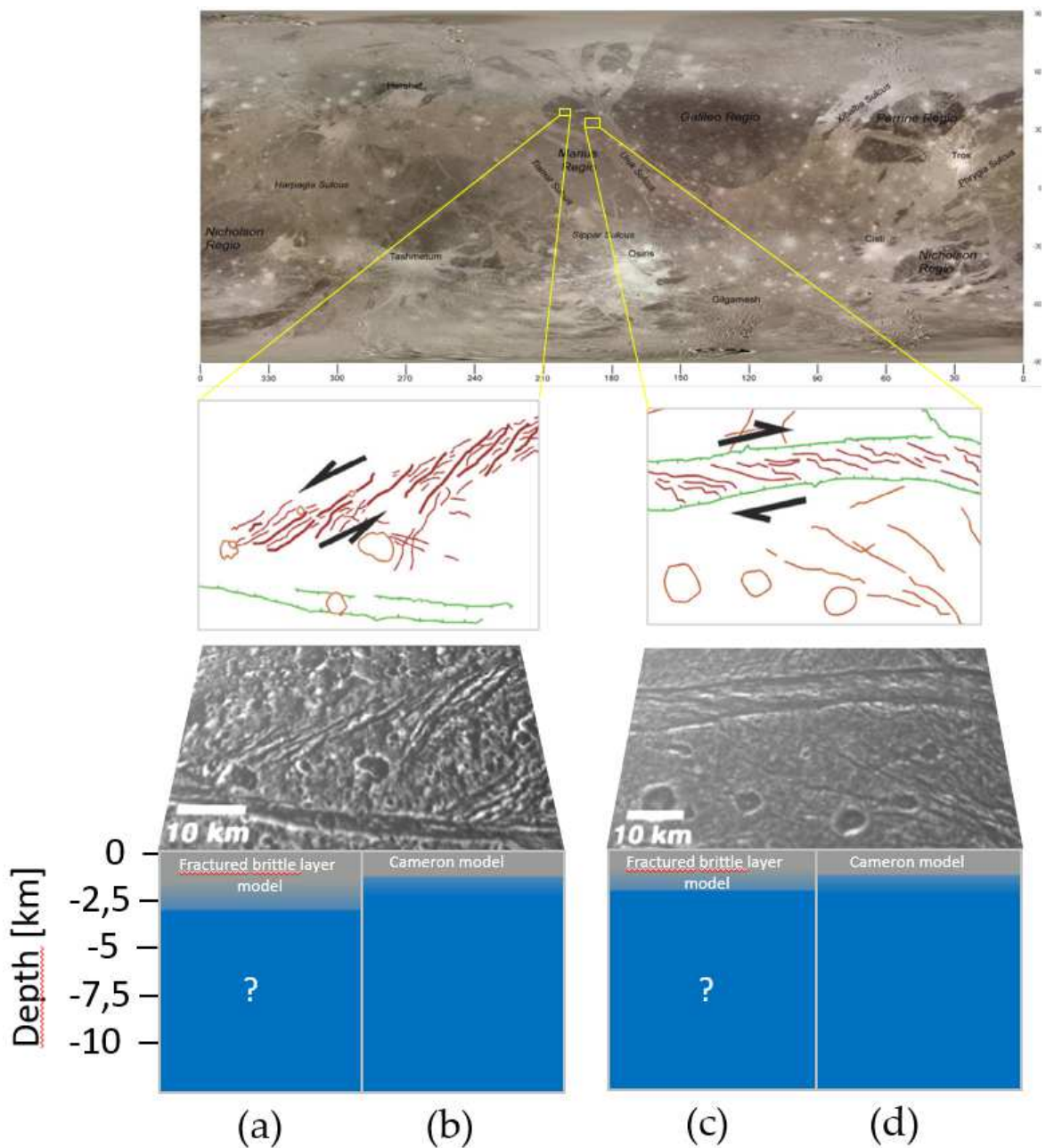
Figure 13. On Top, Ganymede global mosaic in Mercator projection (NASA/ESA/JPL/SSI/Cassini Imaging Team). Bottom left: En-echelon structures within the dark lineated terrain of Anshar Sulcus (162°E, 18°N); In Gray the thickness predicted by Equation 8 (a) vs. the prediction given by Cameron et al., (69-2019) (b). Bottom right, en-echelon structures in the light subdued material found within Transitional Terrain (173°E, 32°N). In Gray the thickness predicted by Equation 8 (c) vs. the prediction given by Cameron et al., (2019) (d). Arrows indicate inferred shear sense assuming a transtensional
