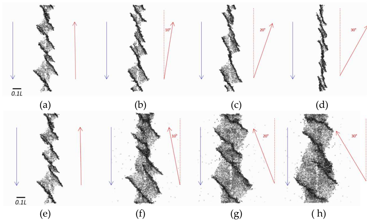
Figure 6. Top views of the numerical models used to simulate the propagation of en-echelon fractures in an intact elastic brittle layer of thickness T_{ref} subjected to transtension (TT for TransTension) modes for different angles \theta_D of divergence with the associated test ID: (a) 0^\circ , PSS_ T_{ref} ; (b) 10^\circ , TT_10; (c) 20^\circ , TT_20 and (d) 30^\circ , TT_30. Bottom views, Transpression (TP) modes are controlled for different angles \theta_c : (e) 0^\circ , PSS_ T_{ref} ; (f) 10^\circ , TP_10; (g) 20^\circ , TP_20 and (h) 30^\circ , TP_30.
