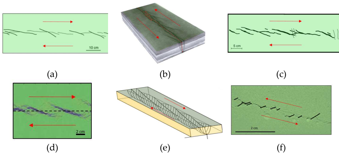
Figure 1. Some experimental models of the formation of en-echelon structures: (a) Sand box model (Naylor et al., 1986); (b) Sand box model (Xiao et al., 2017); (c) Clay model (Atmaoui et al., 2005); (d) Sand box model (Lefevre et al., 2020); (e) Sand box model (Ueta et al., 2000); (f) Gypsum model (Goldstein and Osipenko, 2012).
