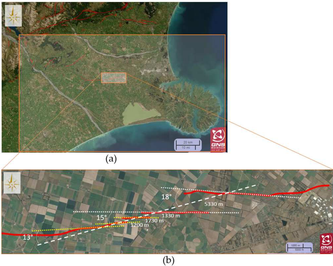
Figure 9. (a) Surface traces of onshore active faults in the Christchurch area with the Eastern section of the Greendale fault (source: GNS science) (b) Spacing distances between the longest en-echelon Riedels identified on the West of the hamlet of Greendale (the distances are measured along the direction of the estimated P shear).
