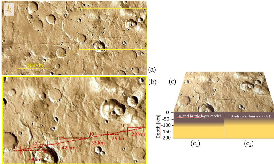
Figure 11. (a) Potential transensional strike-slip fault along a Graben zone in the Memnonia region to the southwest of Tharsis ( 13^{\circ}52'29.25''S , 160^{\circ}39'18.19''O ), West of Burton crater (Image NASA/USGS/DLR/FU Berlin). (b) The spacing distance between the en-echelon segments oriented along the dash line with the associated twist angles). (c) In dark brown, the estimated brittle crust thickness of 72-101 km predicted by Equation 8 ( C_1 ). Also in dark brown, the crustal thickness 35 and 100 km estimated by Andrews-Hanna et al. (2008) based on thermal evolution models ( C_2 ). Note that the gradient between two colors indicates the level of uncertainty.
