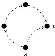
Figure 3: Illustration of a fractional solution satisfying constraints (4) and violating constraints (5): all represented arcs are associated with 0.5 valued variables, the dashed path uses channel {1} and the dotted path uses channel {2}.
