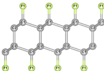
Fig. 5 Crystal structure of a “F-diamane”-like (C_2F) monolayer.
