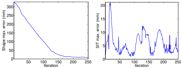
Fig. 8. Shape servoing results. Left: maximum (among all particles) servoing error measured as the difference between the current and the desired shape. Right: maximum (among all particles) error of shape tracking w.r.t. the ground truth for the current shape.
