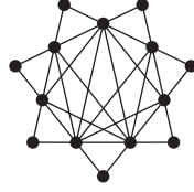
Figure 7: A chordal coordinated odd sun.
