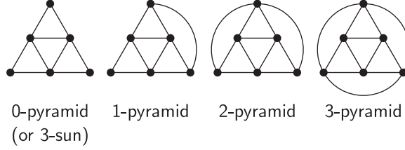
Figure 3: From left to right: 0-, 1-, 2- and 3-pyramid
