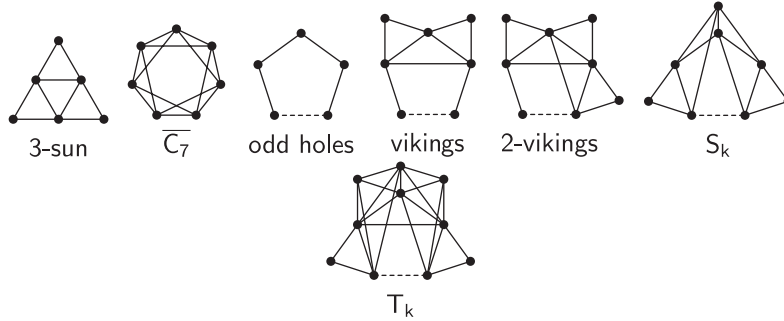
Figure 10: Minimal forbidden induced subgraphs for clique-perfect graphs inside the class of Helly circular-arc graphs. Dashed lines represent induced paths of length 2k - 3 for each k \geq 2 .
