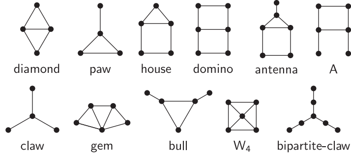
Figure 1: Some small graphs
