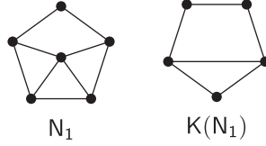
Figure 2: The graph N_1 and its clique graph
