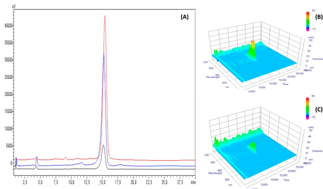
Figure 5. (A) Chromatograms at 408 nm amphotericin B solubilised in 2-hydroxypropyl- \gamma -cyclodextrins (diluted 1/100th to the theoretical concentration of 25 \mu\text{g}/\text{mL} ) at day 0 (red curve), after 168 days at 5 ^{\circ}\text{C} storage (blue curve) and 25 ^{\circ}\text{C} (black curve); with diode array detector screening after 168 days at 5 ^{\circ}\text{C} (B) and at 25 ^{\circ}\text{C} (C). \mu\text{V} and mAU: units of intensity of signal measured by the UV-visible detector.
