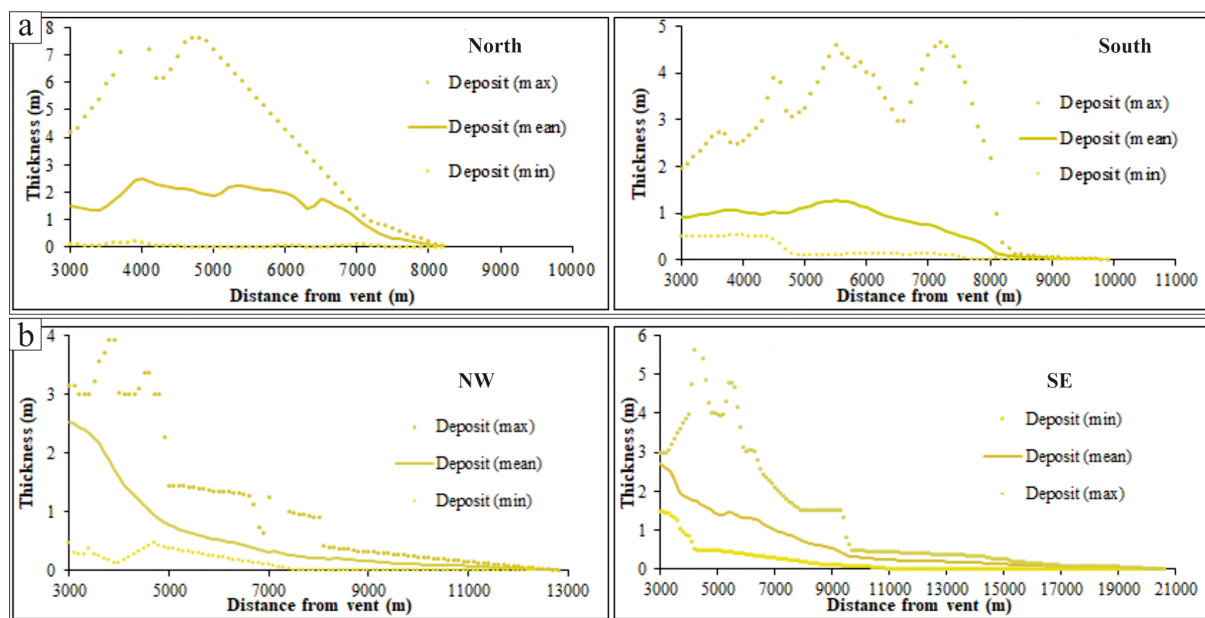
Figure B1. Deposit thickness for (a) EU3pf and (b) EU4b/c units. “Max”, “Mean” and “Min” refer to, respectively, the maximum, mean and minimum thicknesses measured along each circle described in Sect. 3.2.
