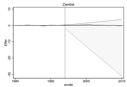
Figure 9: Synthetic control. vs Demeaned synthetic control (6)
