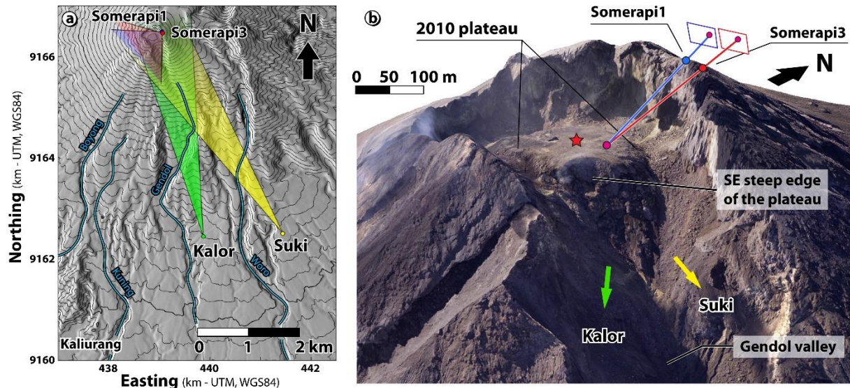
Fig. 1 (a) Location of the four monitoring stations at Merapi volcano and the Gendol river. (b) 3D view of the summit before the birth of the dome, with the locations of the summit monitoring stations. The red and blue lines indicate how a point is localized in 3D by stereophotogrammetry. The red star indicates the vent location of the 2018 lava dome
