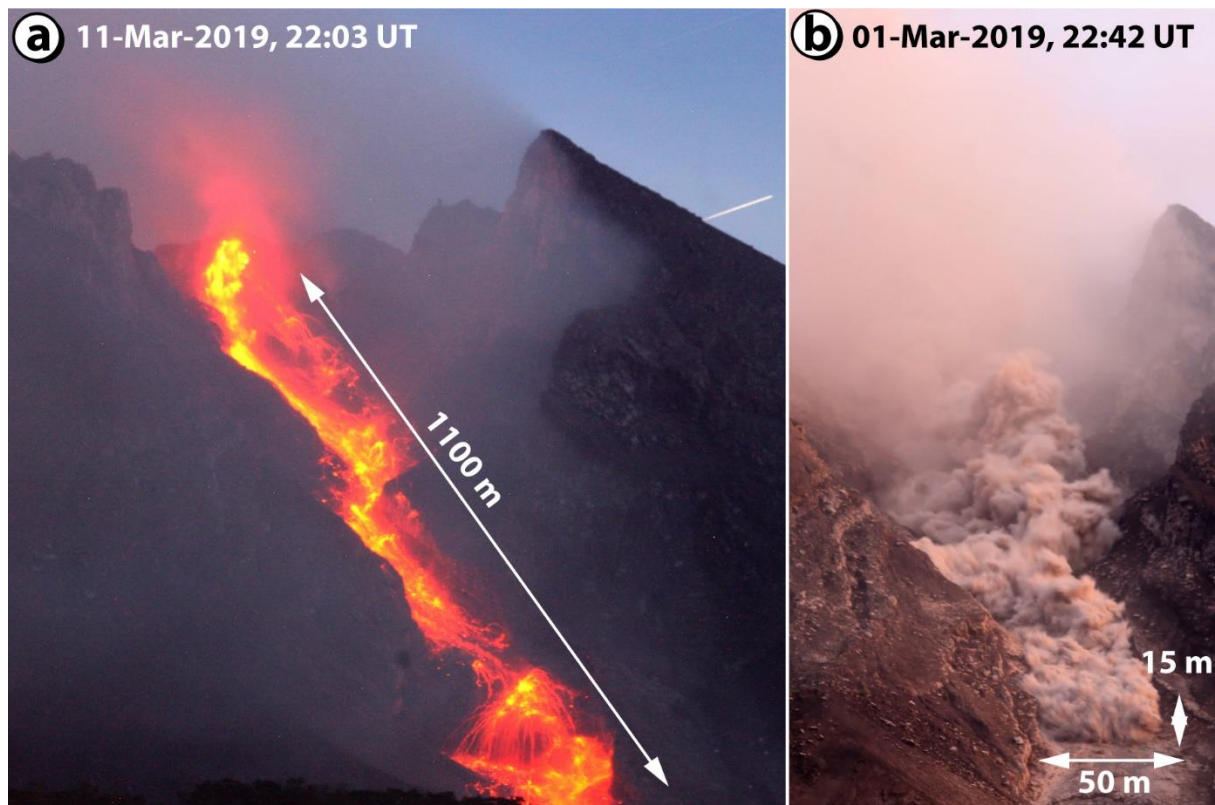
Fig. 9 (a) Pyroclastic flow recorded by night. The long duration of the exposure (600 s) makes it possible to see block trajectories through the companion ash-cloud. (b) A companion ash-cloud recorded during the day
