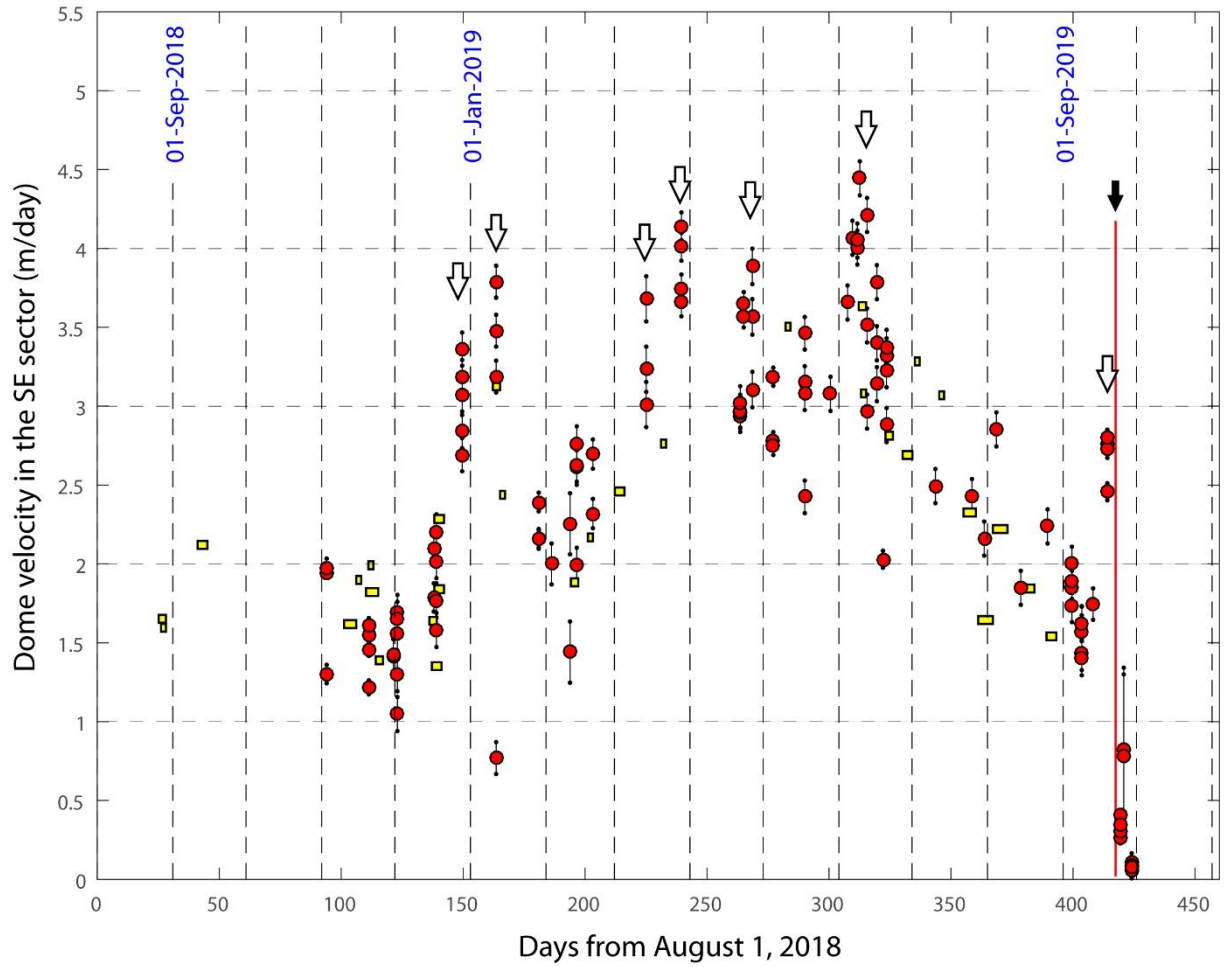
Fig. 5 Evolution of the surface velocities of the lava dome in the SE sector. The red circles are velocities calculated from visible images and the yellow rectangles from the thermal camera. The arrows indicate periods of higher flow velocities associated with a major collapse. The red line marks the explosion of 22 September 2019 and the end of the dome emplacement
