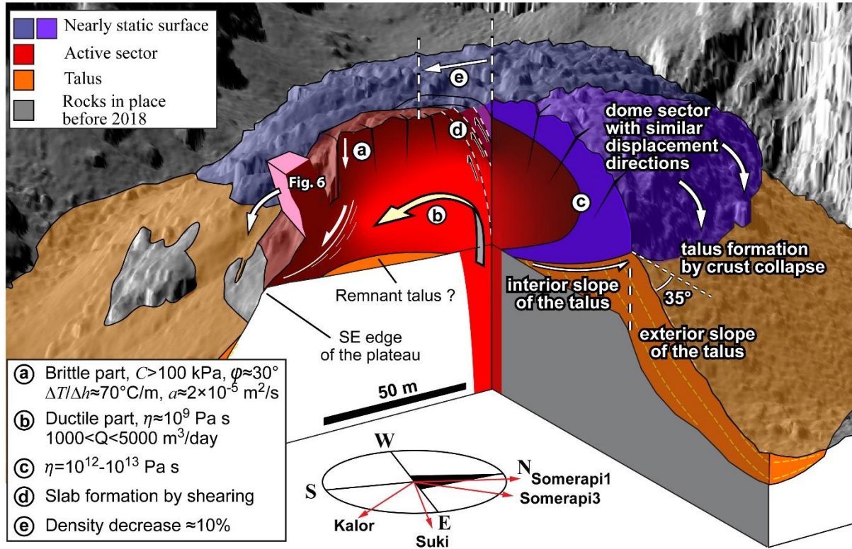
Fig. 4 Summary sketch of the observations and the interpretations of the dome emplacement (the dome morphology is that of July 2019 but some features appeared before, during phase 2 and early phase 3)
