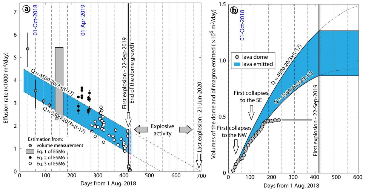
Fig. 8 (a) Effusion rate with time. The colours of the symbols are related to the method used (see ESM-7 for the equations of the effusion rates from velocities). The blue area corresponds to a linear evolution of the effusion rate between Q = 3500 - 20/3 \times t and Q = 4500 - 20/3 \times t (b) Volume of the lava dome and cumulated volume of lava emitted with time based on the equations used in (a)
