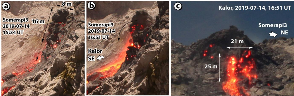
Fig. 6 Close-up photos of the front of the active lava dome showing the type of collapse that generated PDCs from December 2018 to September 2019. (a)–(b) view from a summit station. (c) view from a flank station. The front location is marked in Figure 4
