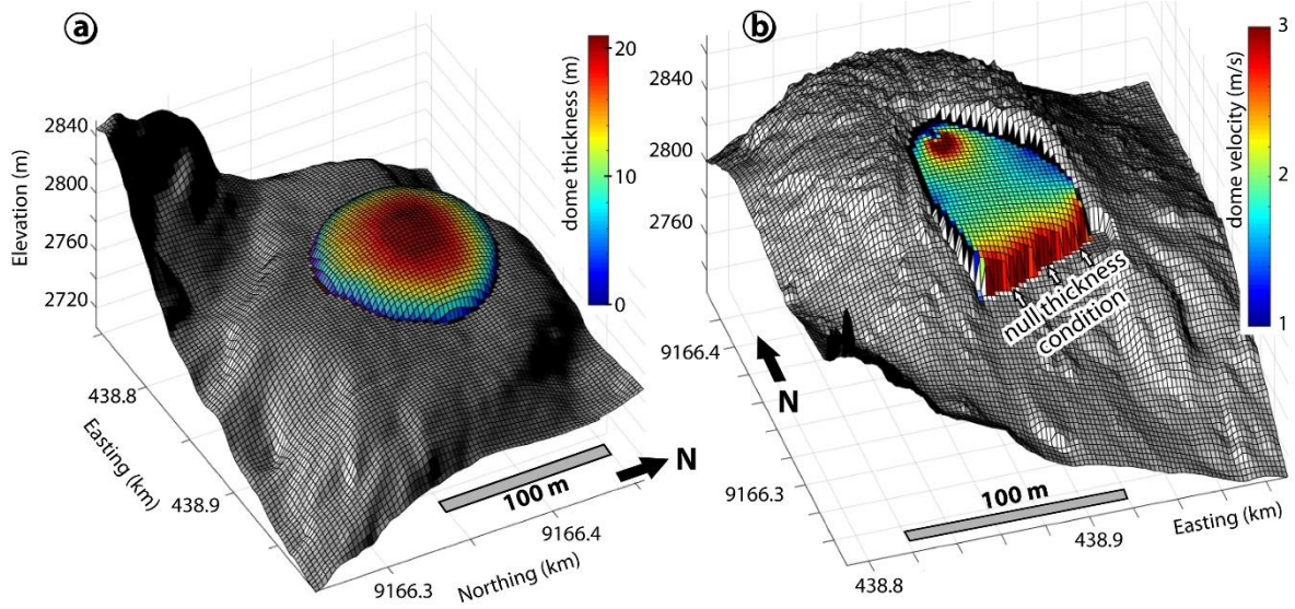
Fig. 7 Simulations of the dome emplacement with VolcFlow (a) Simulation of the 1 st month on the 2010 plateau, with a viscosity of 5 \times 10^{10} Pa s, a density of 2300 \text{ kg/m}^3 and an effusion rate Q = 4000 - 20/3 \times t \text{ m}^3/\text{day} after 30 days. (b) Simulation of the dome emplacement in the SE sector of the new dome (with a viscosity of 10^{11} Pa s, a constant effusion rate of 3000 \text{ m}^3/\text{day} and a null thickness condition imposed at the front of the dome - white arrows)
